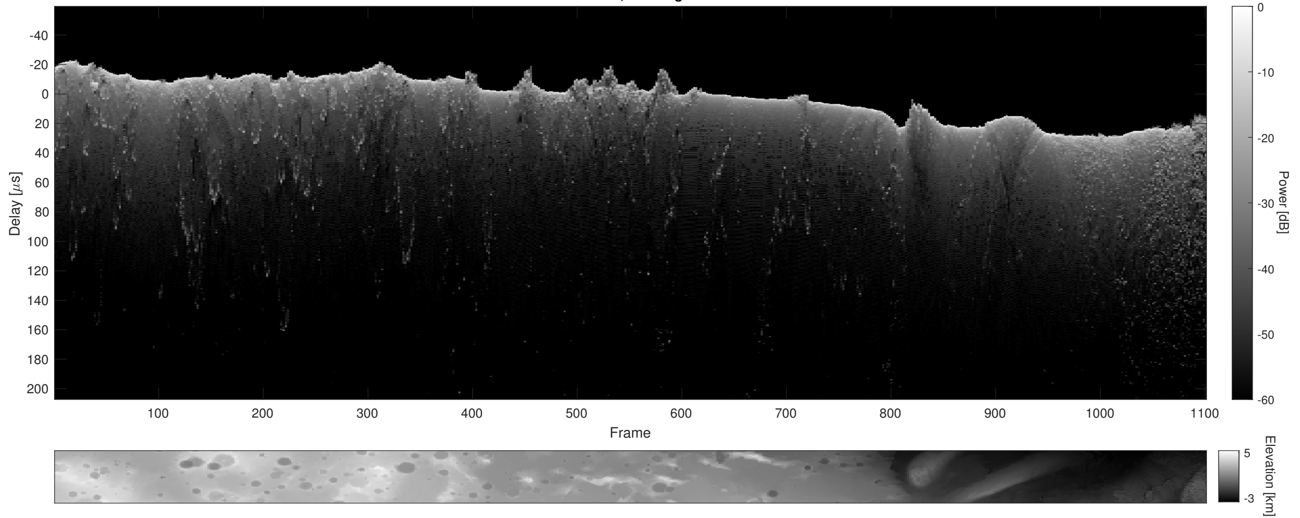
Orbit 2179, Cluttergram
