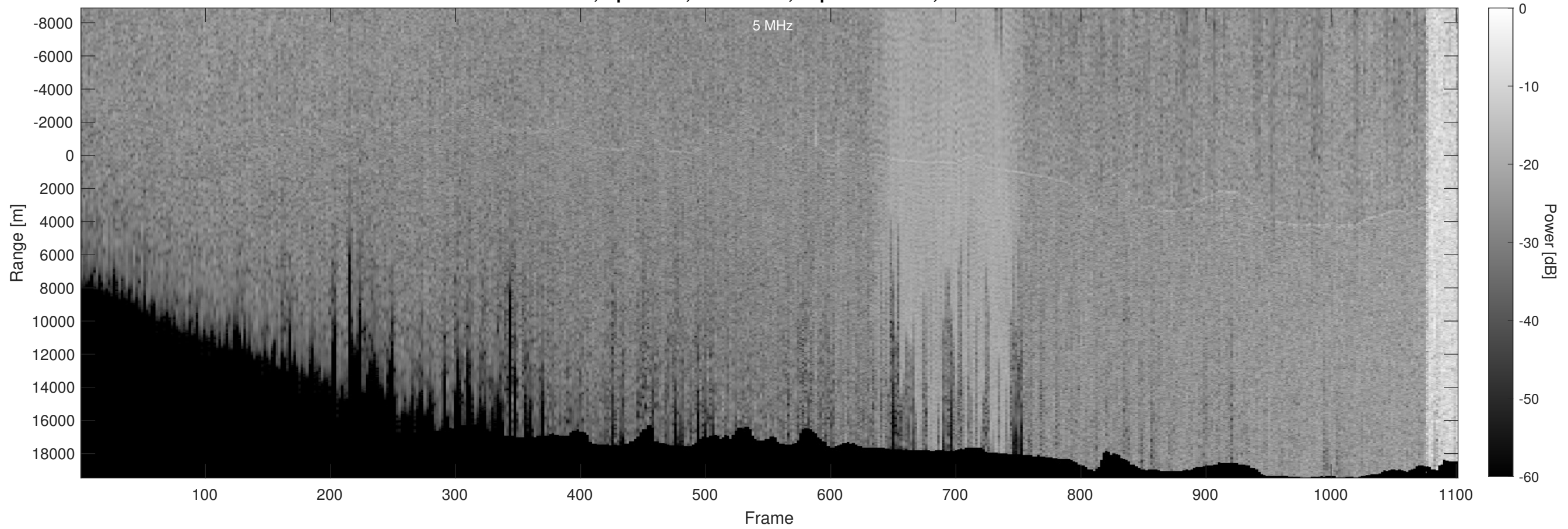
Orbit 2179, Optimized, No Window, Depth-Corrected, Channel 2
