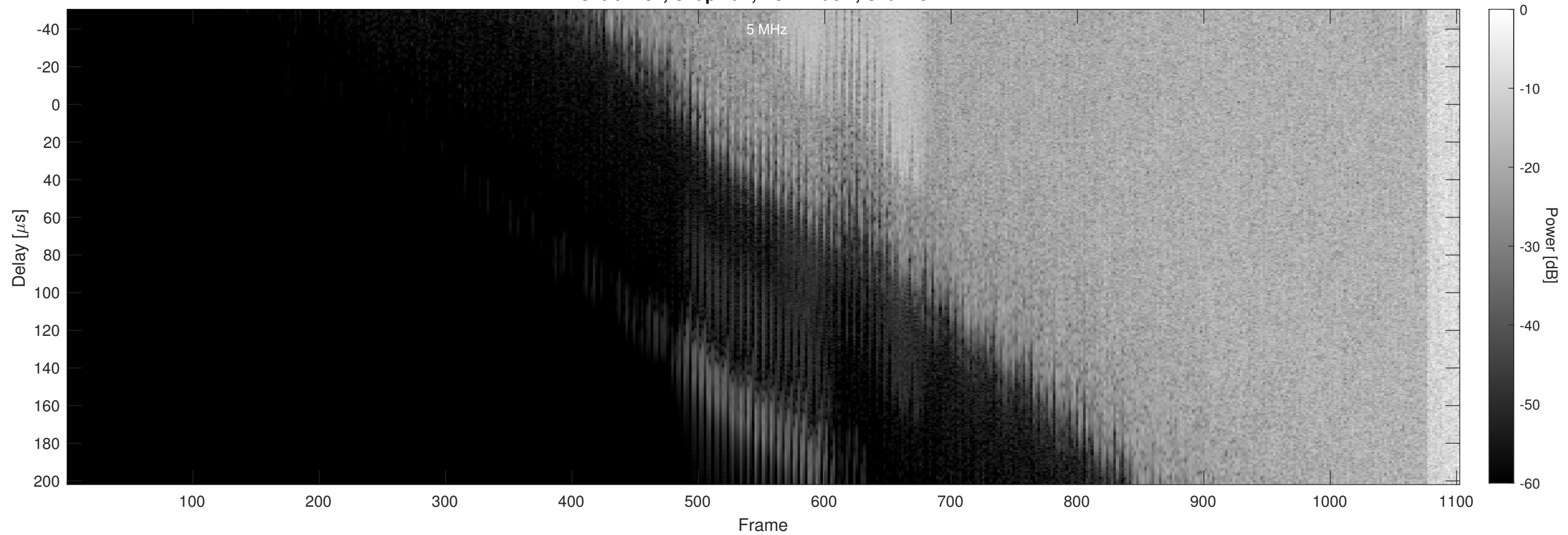
Orbit 2181, Chapman, No Window, Channel 2
