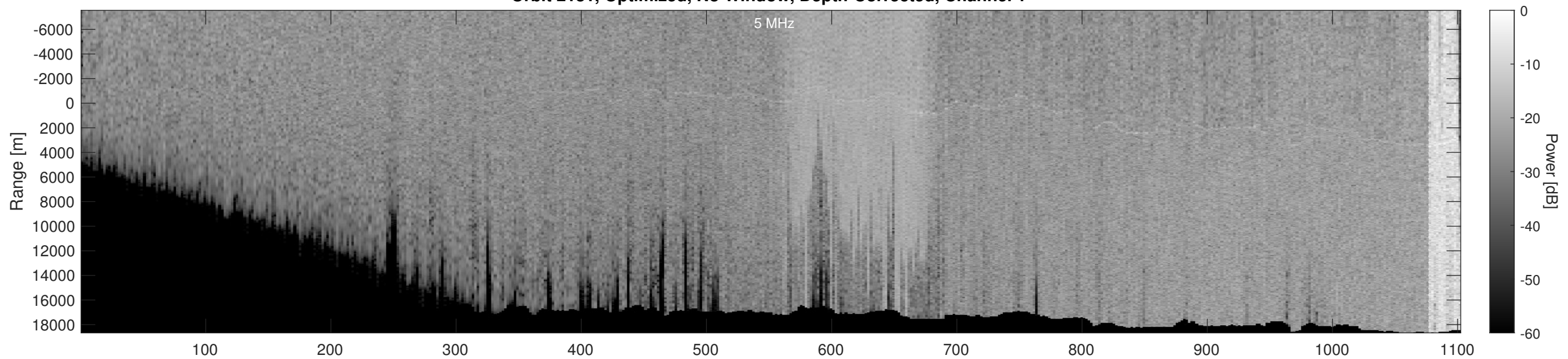
Orbit 2181, Optimized, No Window, Depth-Corrected, Channel 2
