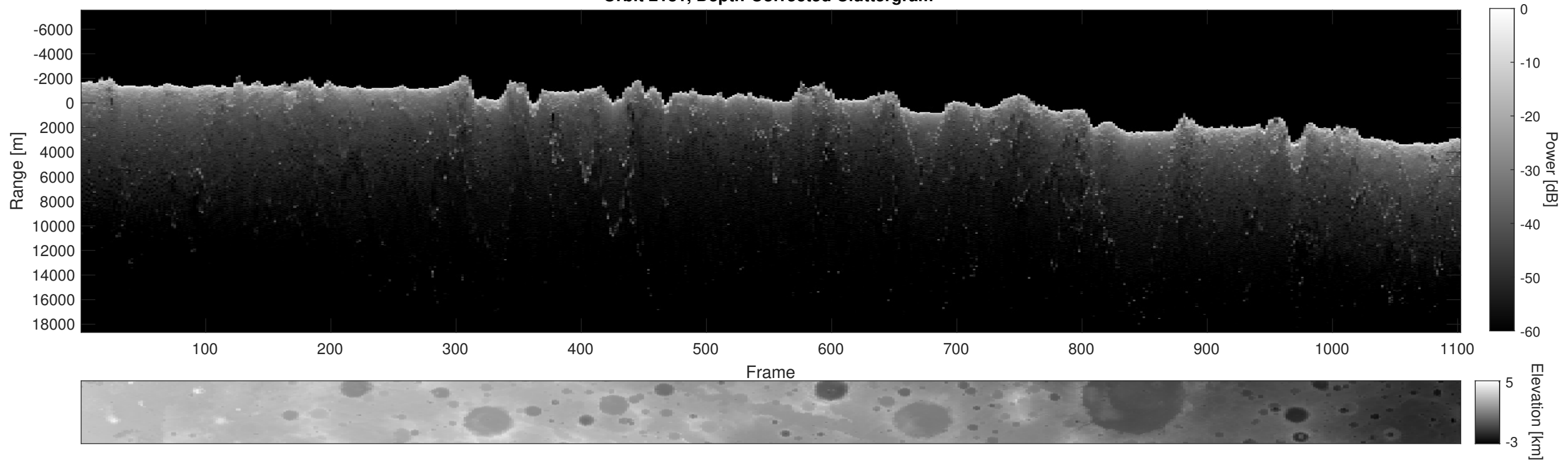
Orbit 2181, Depth-Corrected Cluttergram
