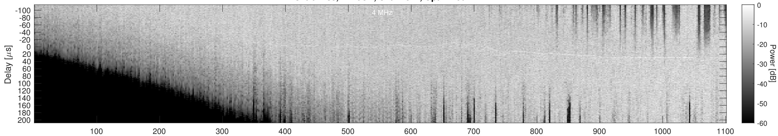
Orbit 2183, Cluttergram
