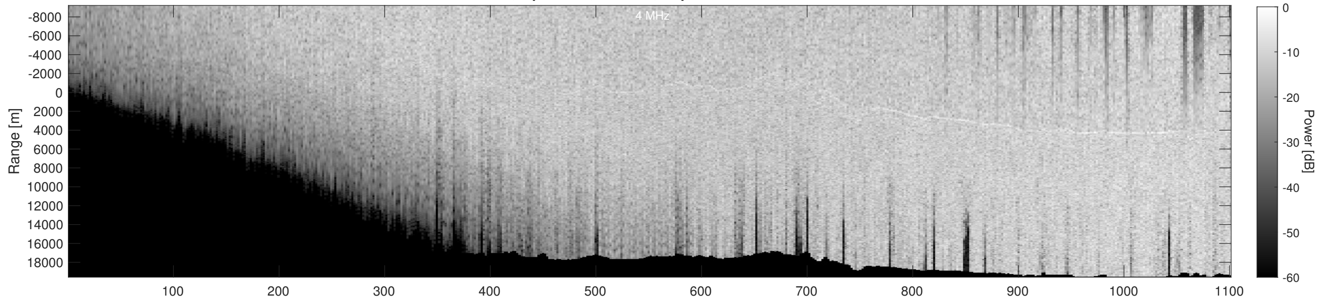
Orbit 2183, Depth-Corrected Cluttergram
