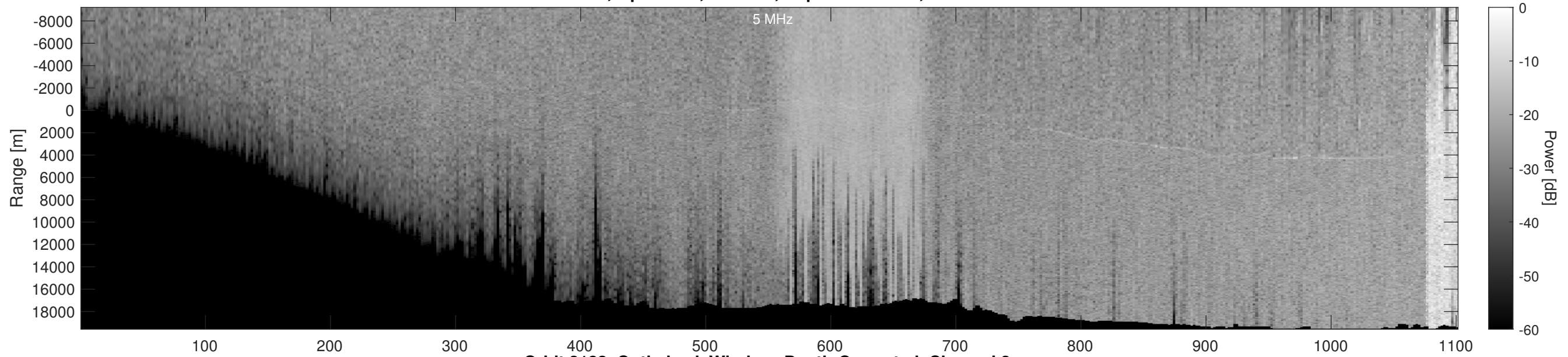
Orbit 2183, Optimized, Window, Depth-Corrected, Channel 2
