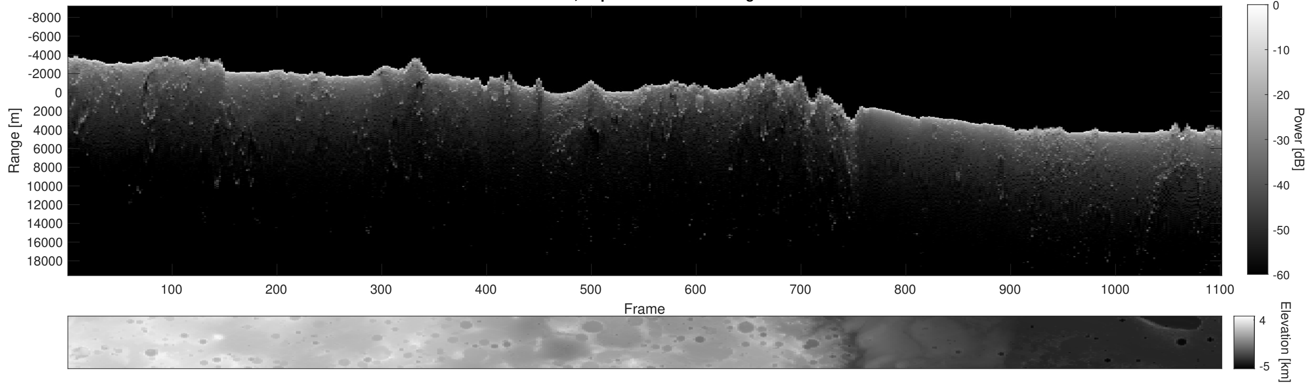
Orbit 2183, Depth-Corrected Cluttergram
