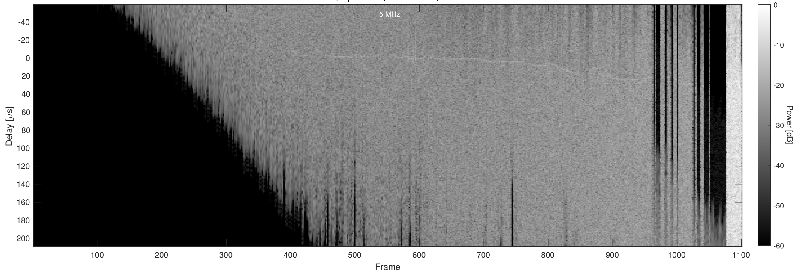
Orbit 2190, Optimized, No Window, Channel 2
