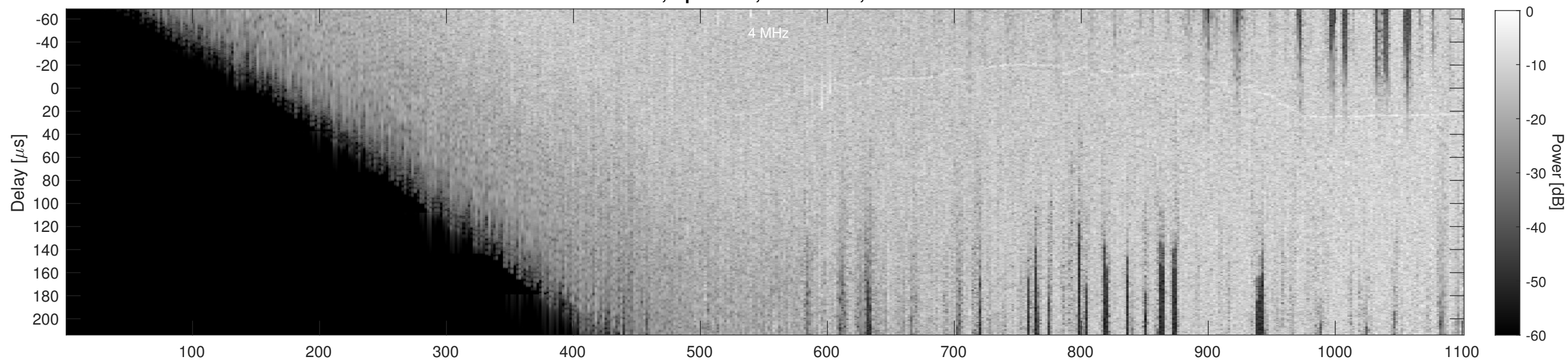
Orbit 2195, Cluttergram
