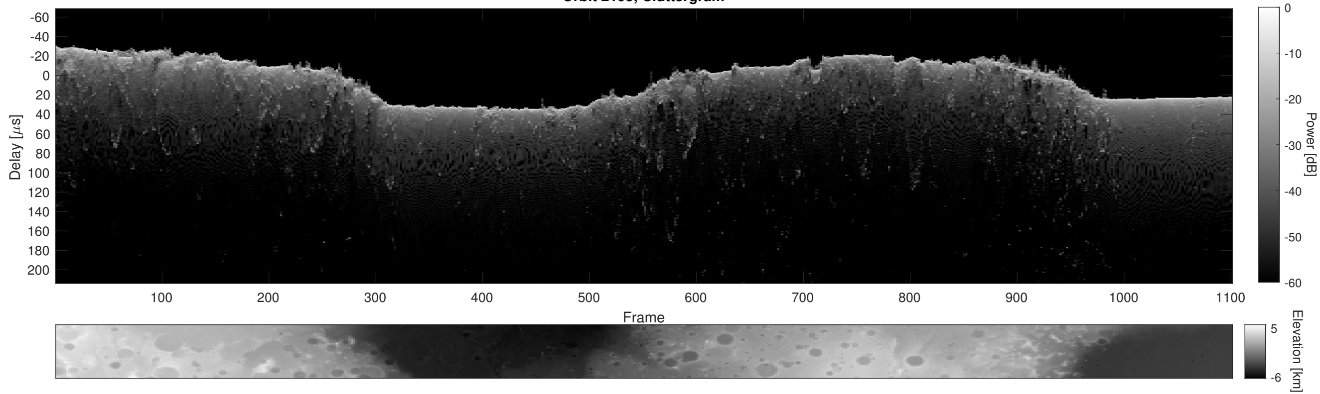
Orbit 2195, Cluttergram
