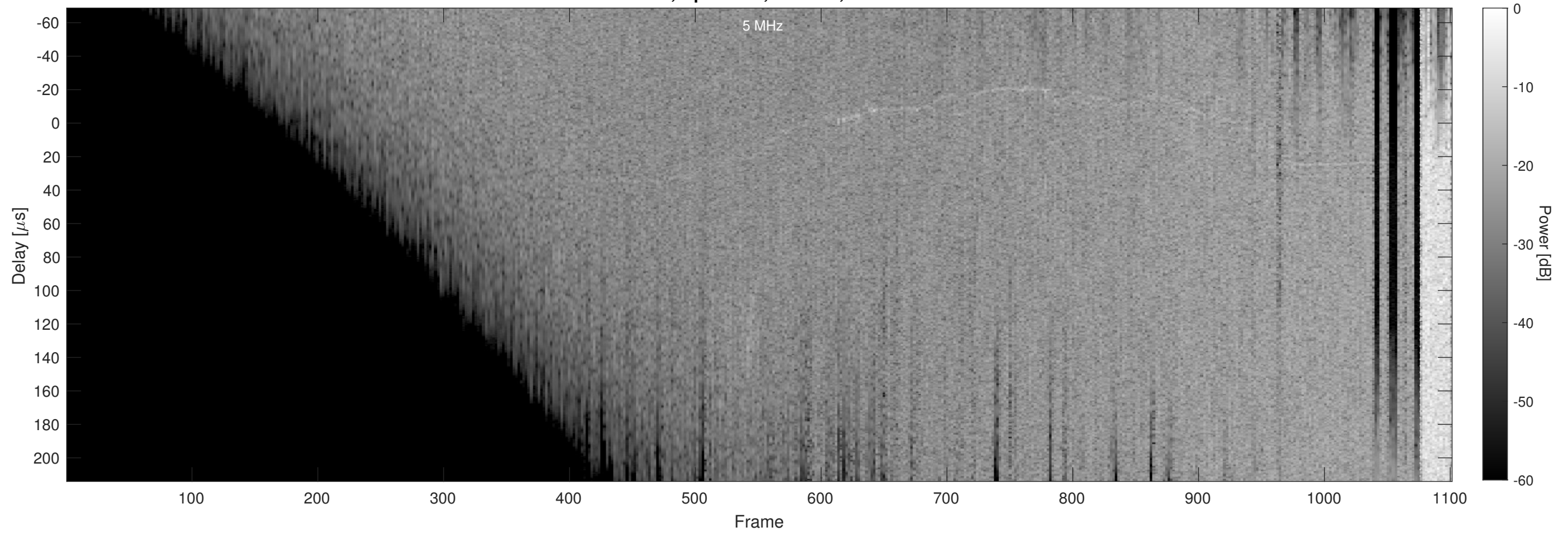
Orbit 2195, Optimized, Window, Channel 2
