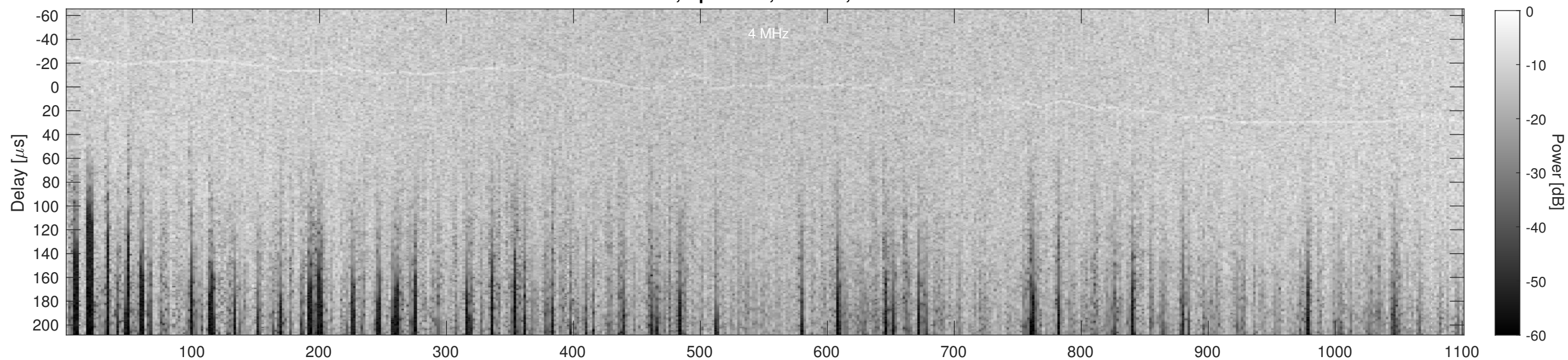
Orbit 2205, Cluttergram
