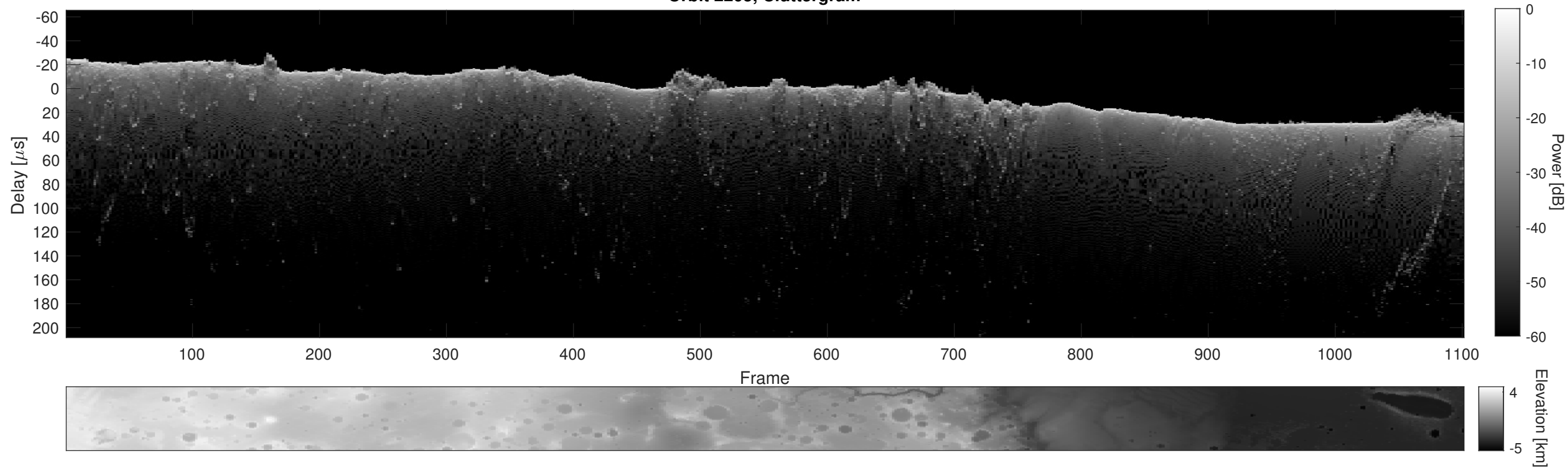
Orbit 2205, Cluttergram
