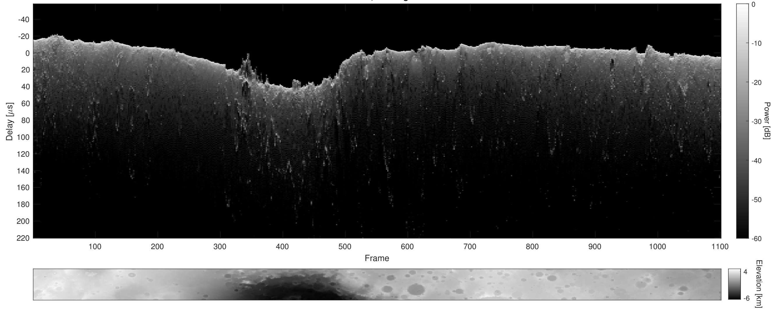
Orbit 2210, Cluttergram
