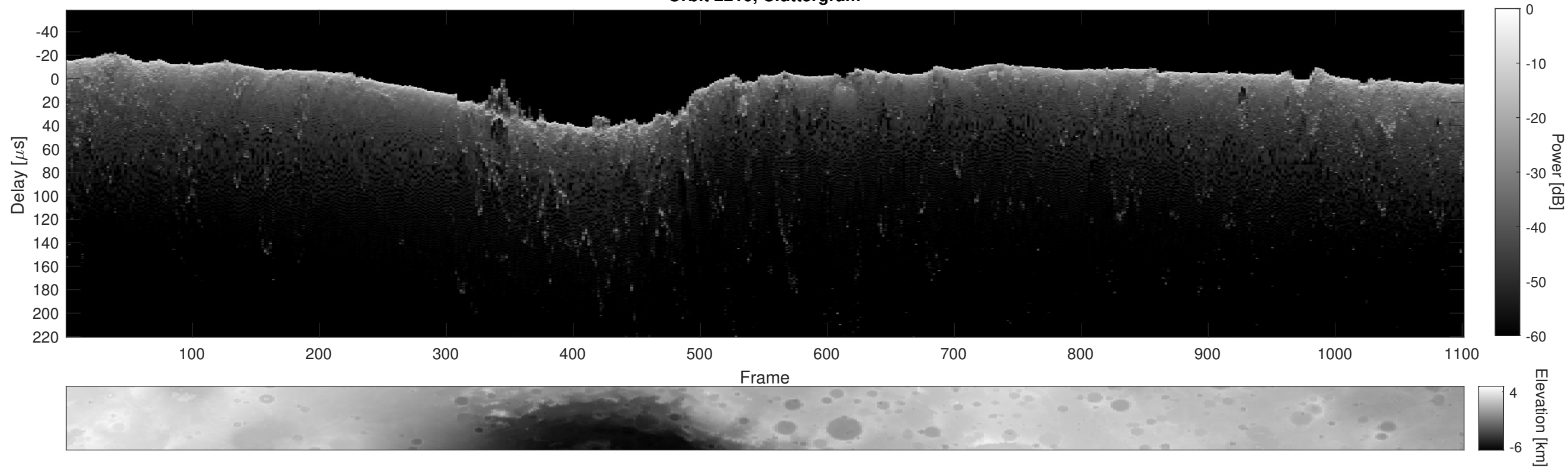
Orbit 2210, Cluttergram
