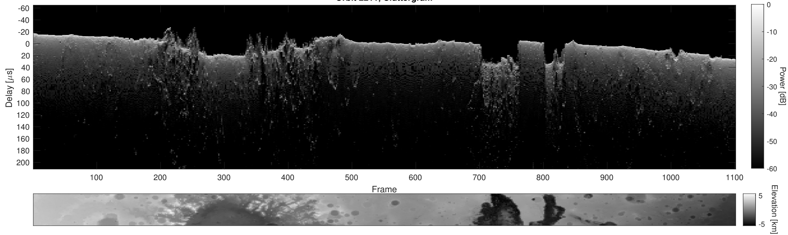
Orbit 2211, Cluttergram
