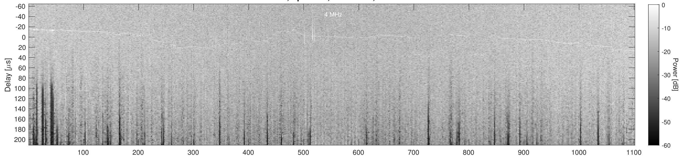
Orbit 2211, Cluttergram
