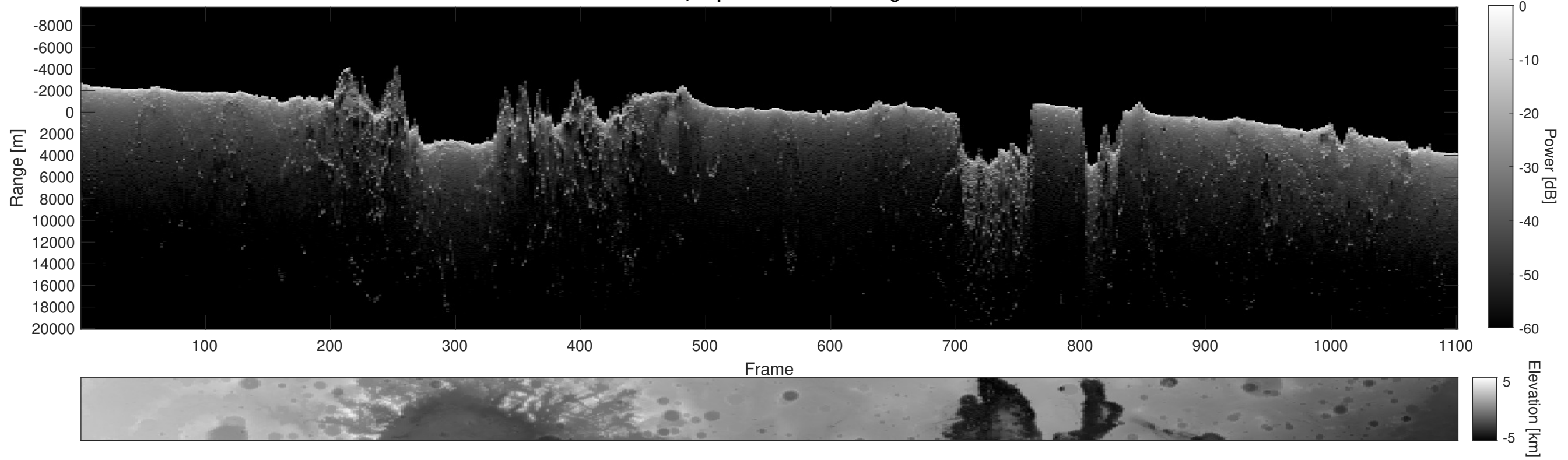
Orbit 2211, Depth-Corrected Cluttergram
