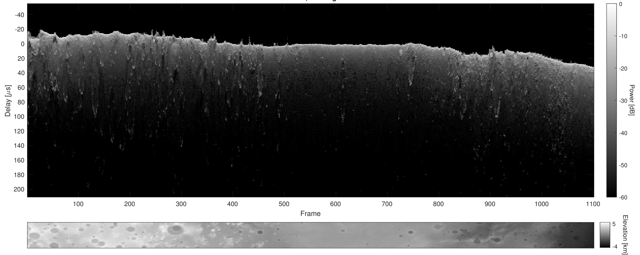
Orbit 2213, Cluttergram
