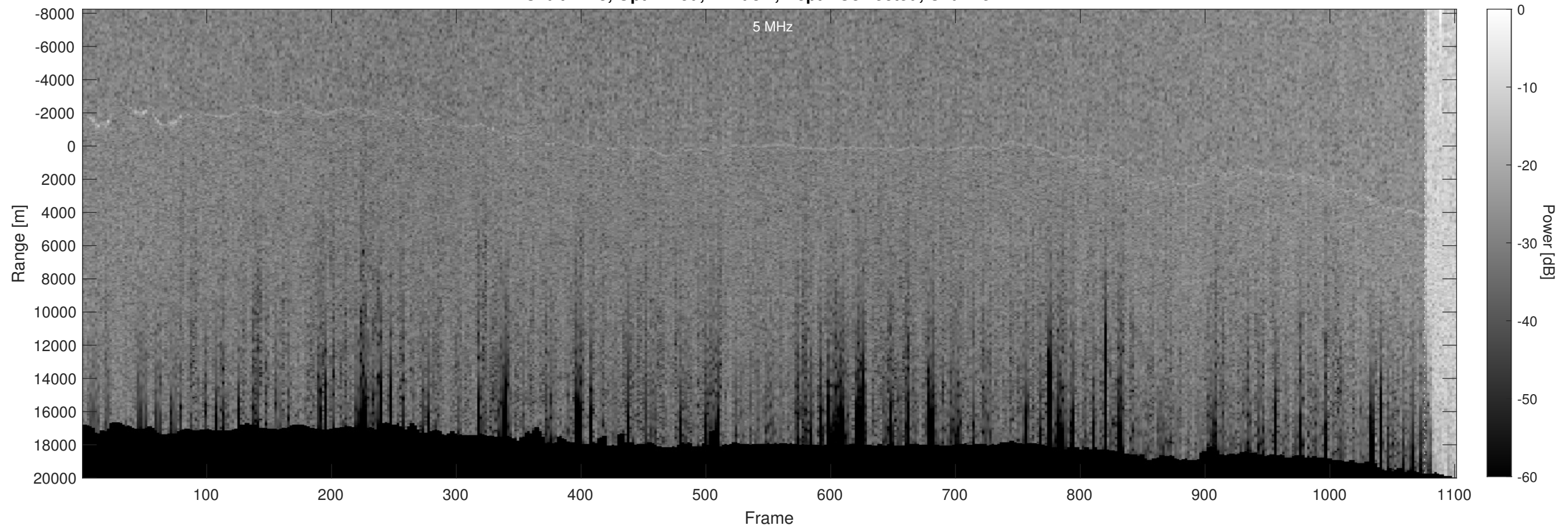
Orbit 2213, Optimized, Window, Depth-Corrected, Channel 2
