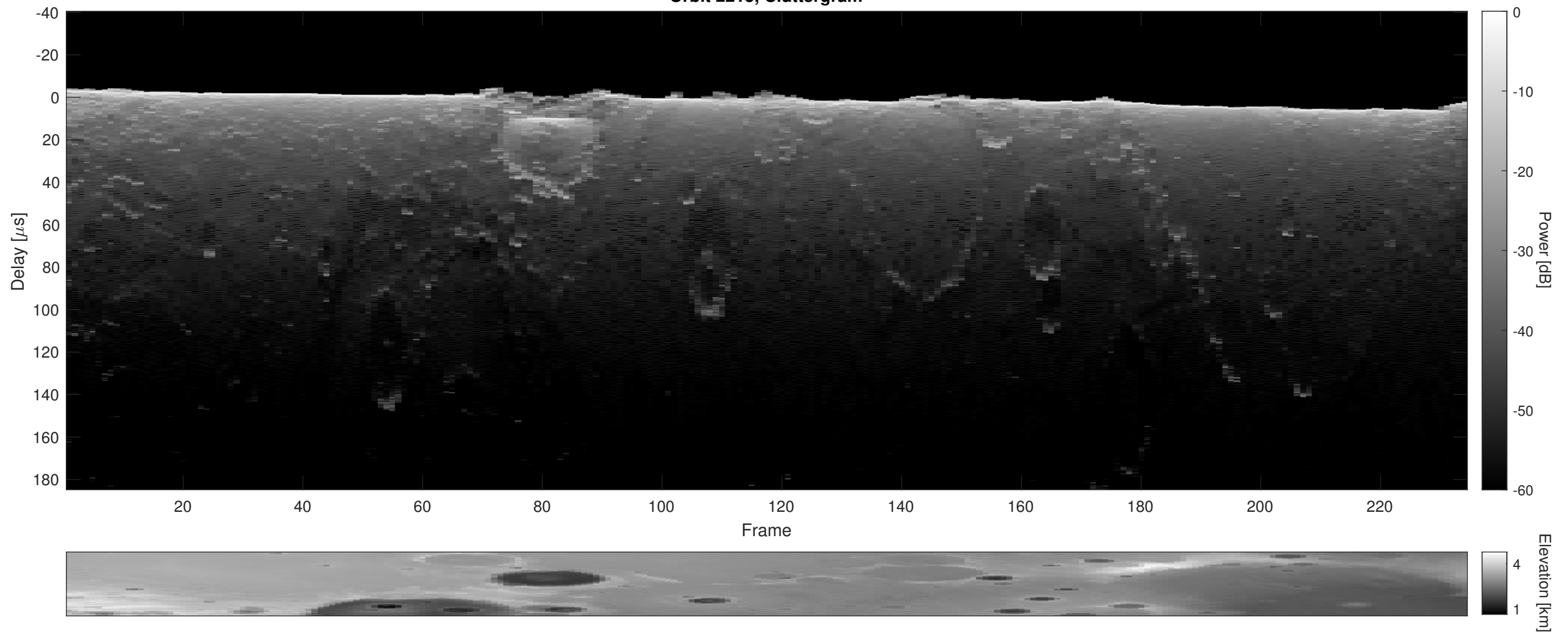
Orbit 2215, Cluttergram
