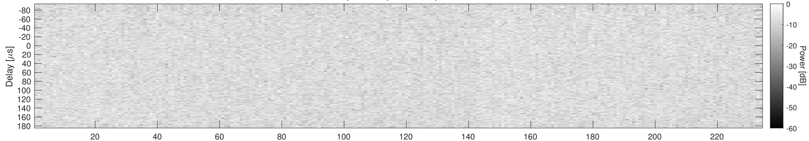
Orbit 2215, Window, Channel 2, Chapman
