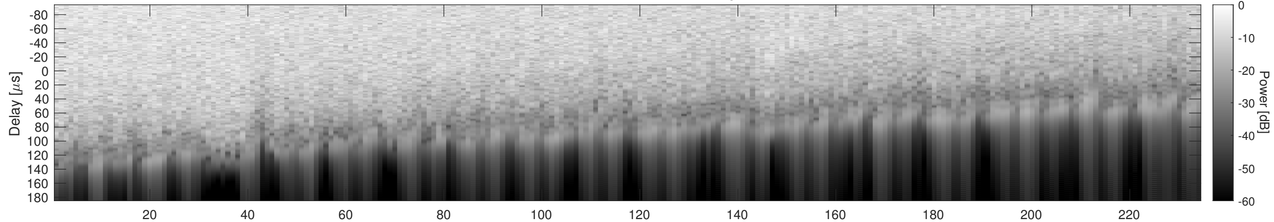
Orbit 2215, Window, Channel 2, Optimized
