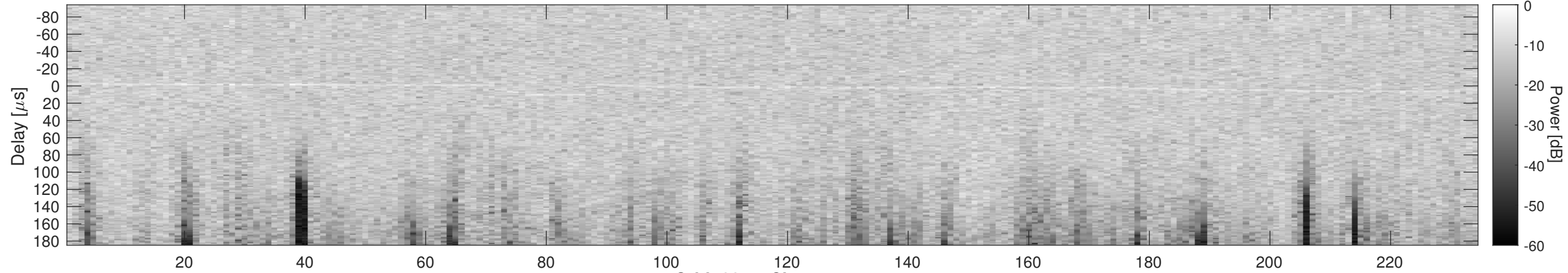
Orbit 2215, Cluttergram
