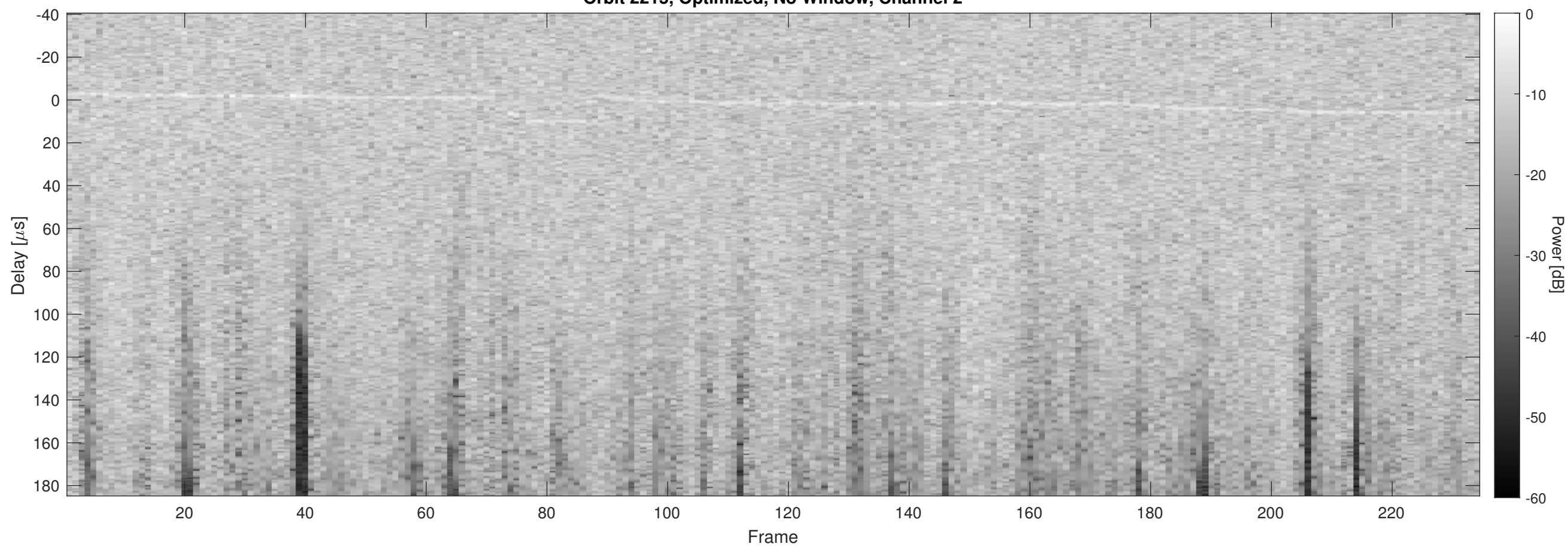
Orbit 2215, Optimized, No Window, Channel 2
