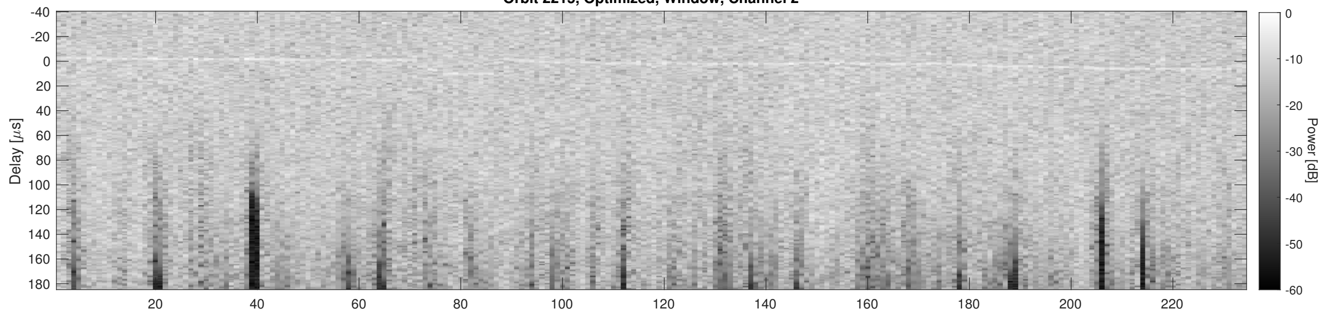
Orbit 2215, Cluttergram
