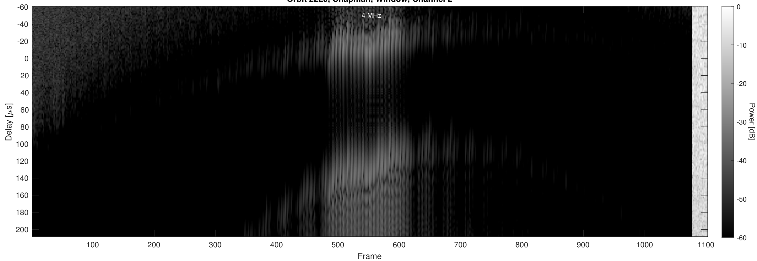
Orbit 2220, Chapman, Window, Channel 2
