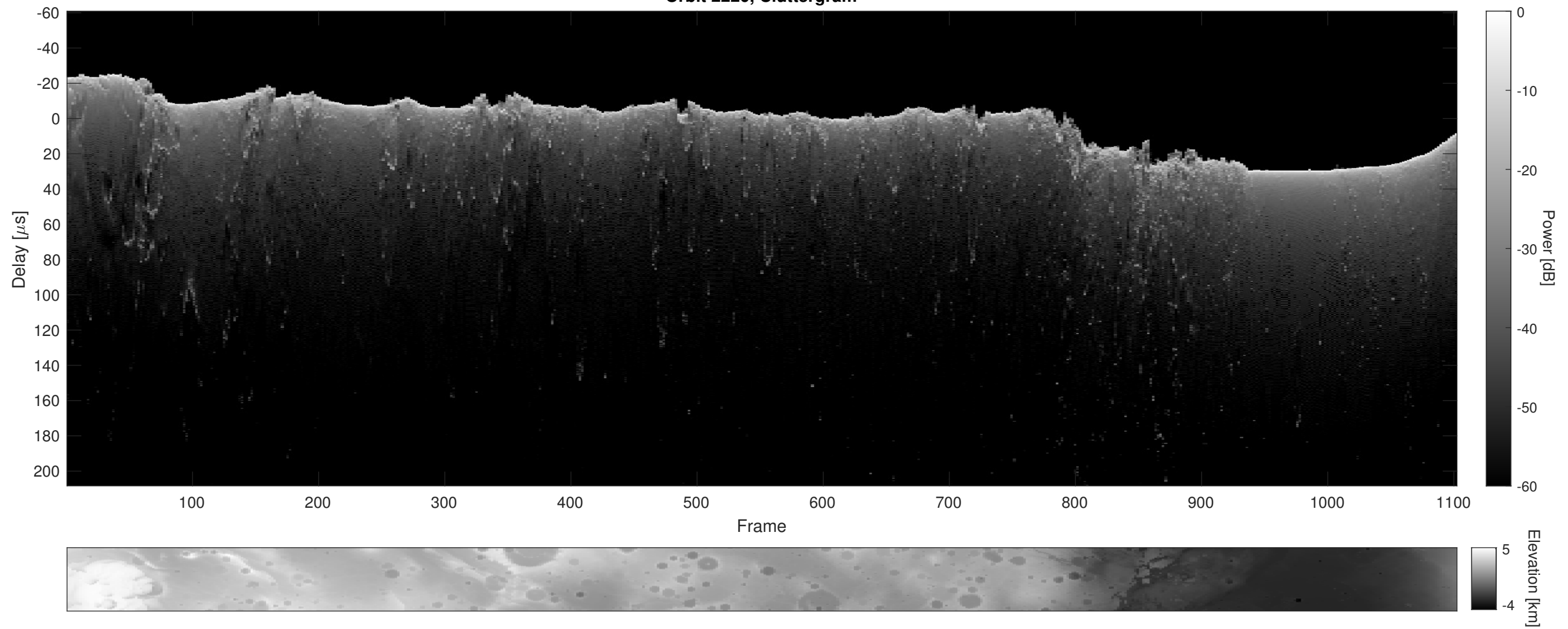
Orbit 2220, Cluttergram
