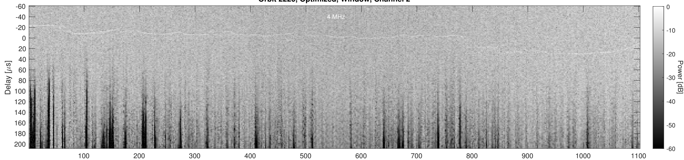
Orbit 2220, Cluttergram
