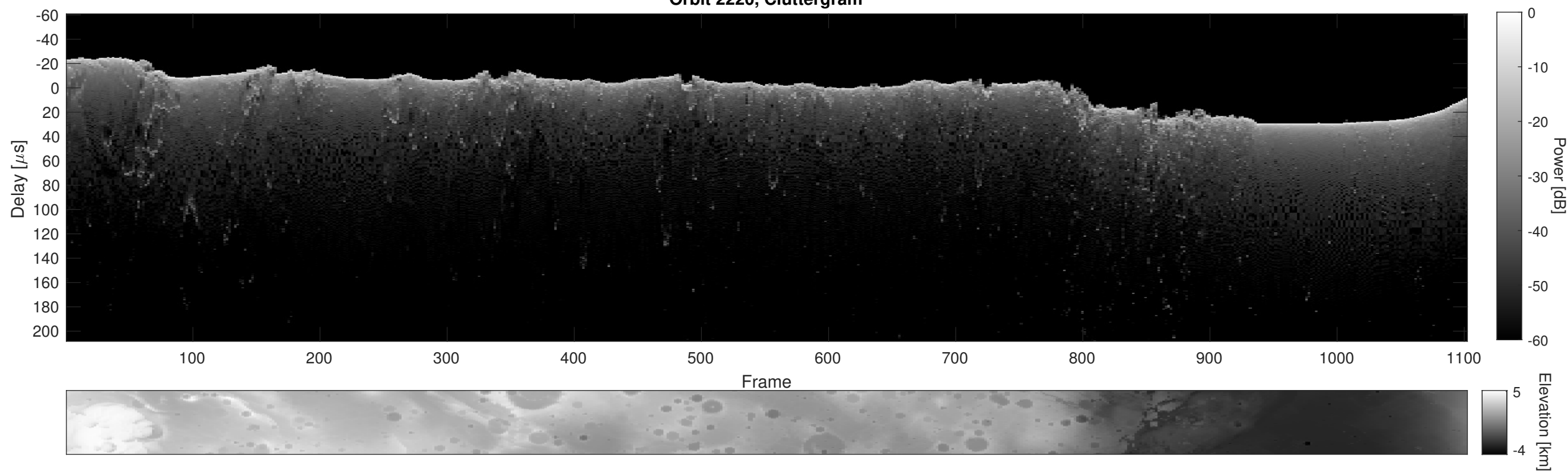
Orbit 2220, Cluttergram
