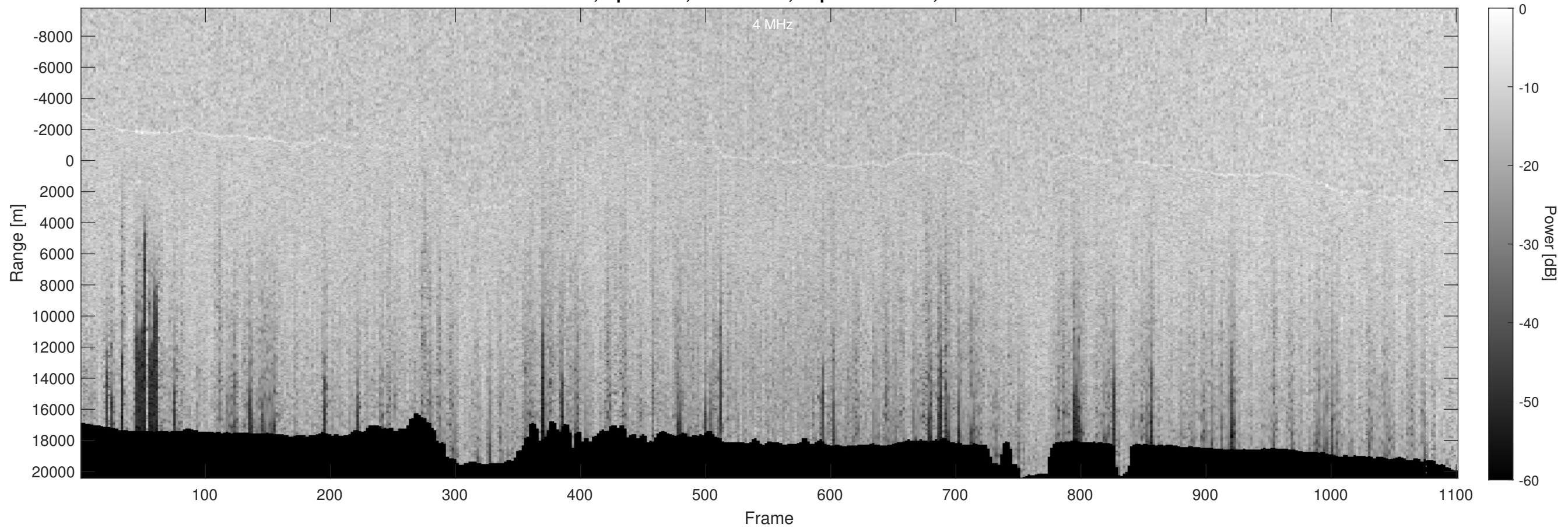
Orbit 2222, Optimized, No Window, Depth-Corrected, Channel 2
