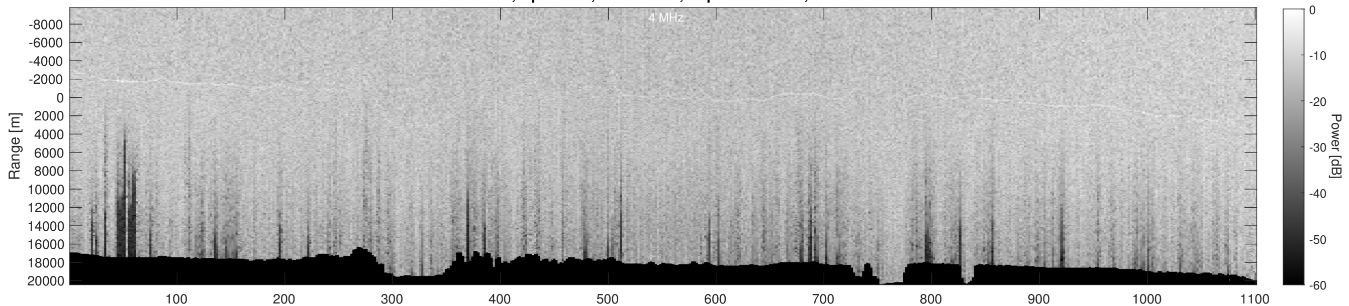
Orbit 2222, Depth-Corrected Cluttergram
