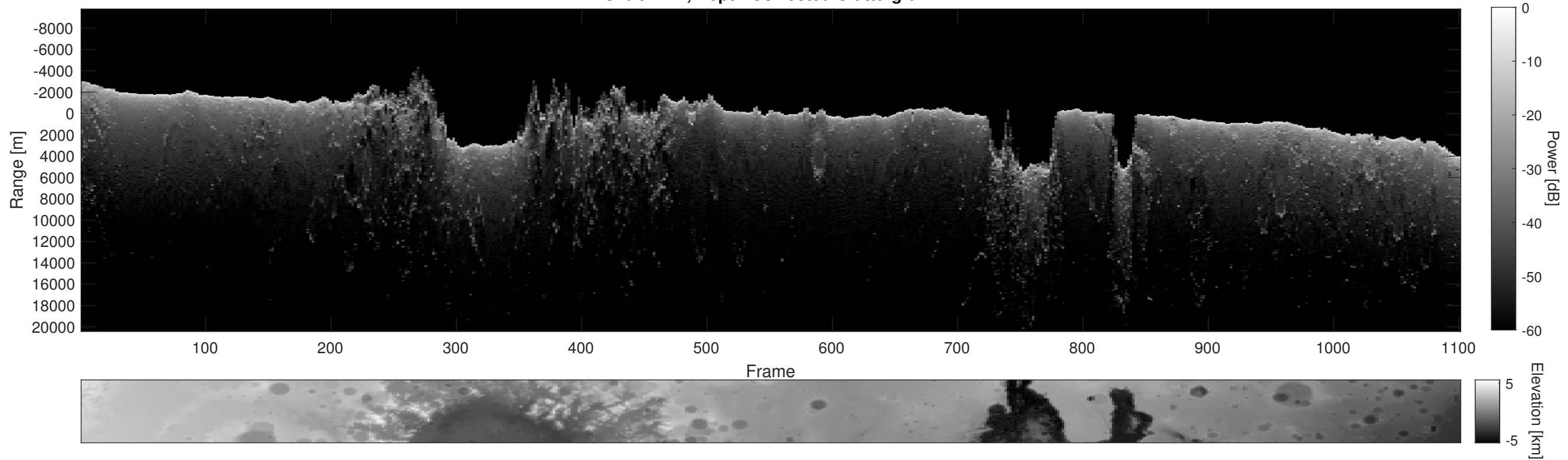
Orbit 2222, Depth-Corrected Cluttergram
