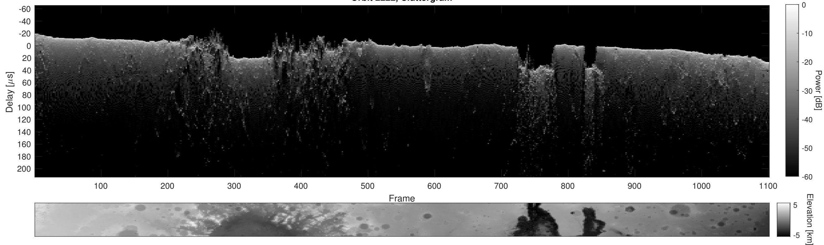
Orbit 2222, Cluttergram
