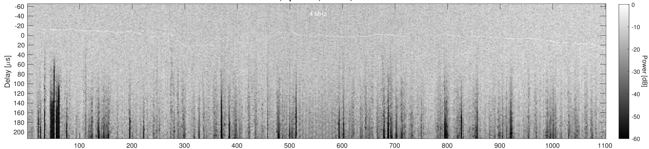
Orbit 2222, Cluttergram
