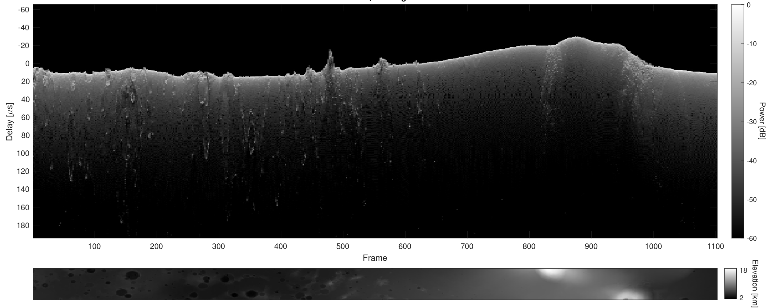
Orbit 2230, Cluttergram
