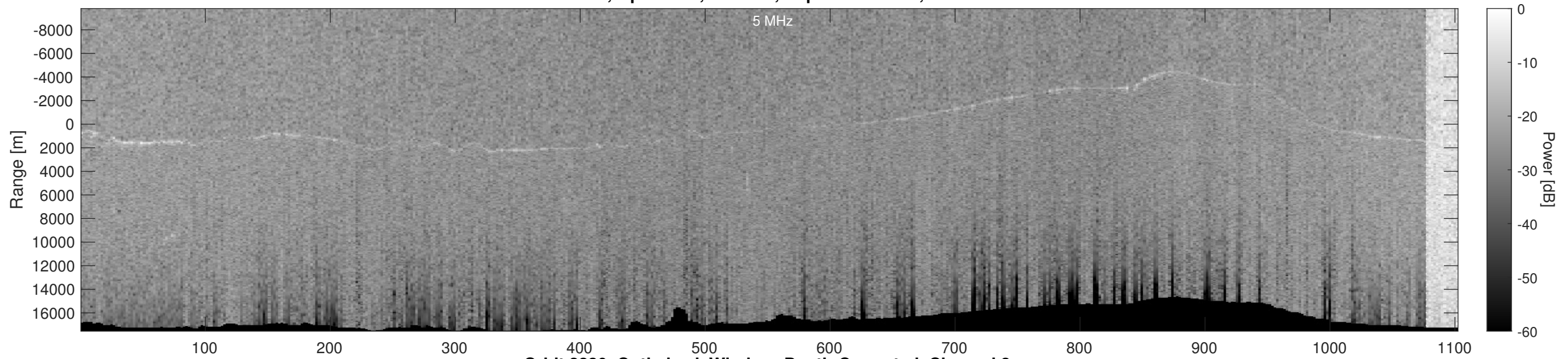
Orbit 2230, Optimized, Window, Depth-Corrected, Channel 2
