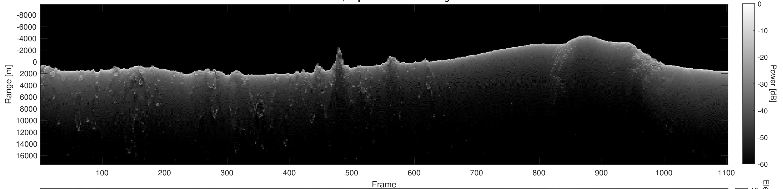
Orbit 2230, Depth-Corrected Cluttergram
