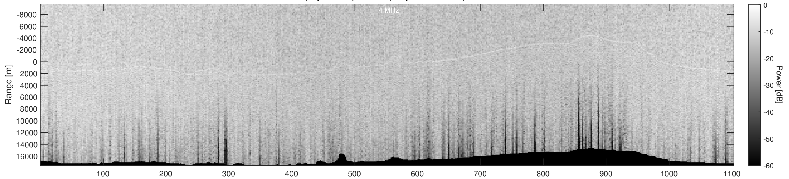
Orbit 2230, Depth-Corrected Cluttergram
