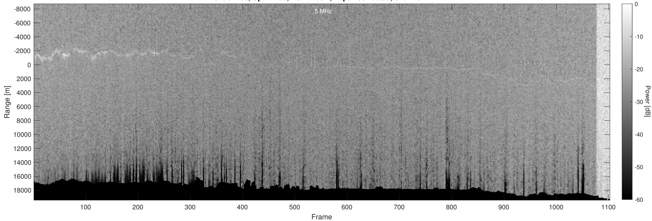
Orbit 2235, Optimized, No Window, Depth-Corrected, Channel 2
