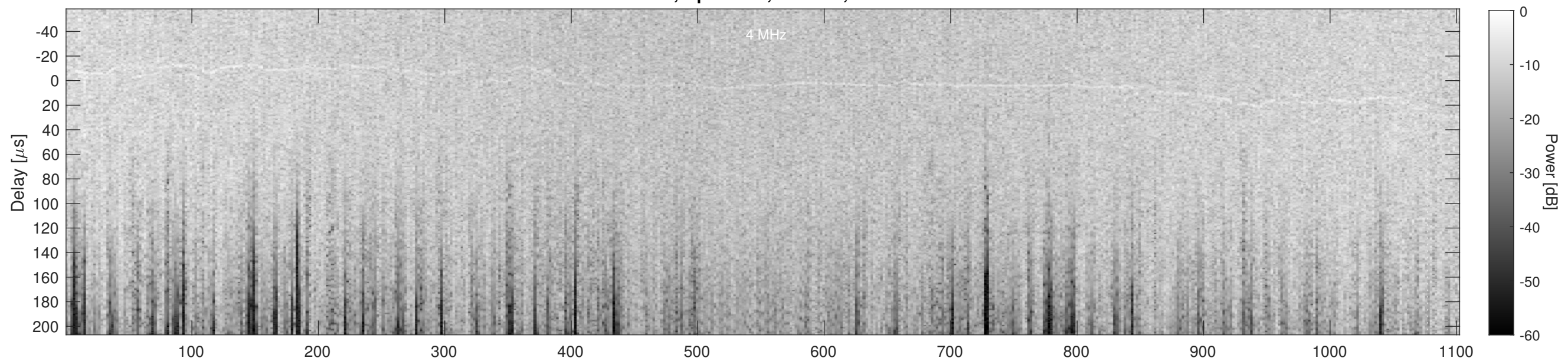
Orbit 2235, Cluttergram
