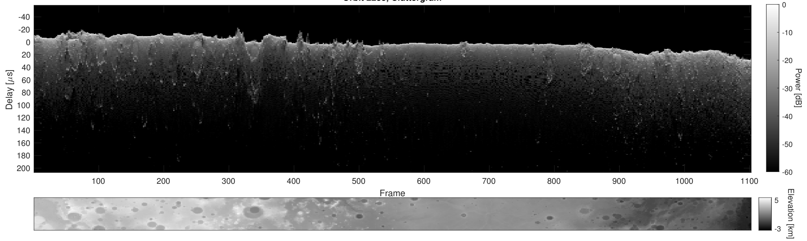
Orbit 2235, Cluttergram
