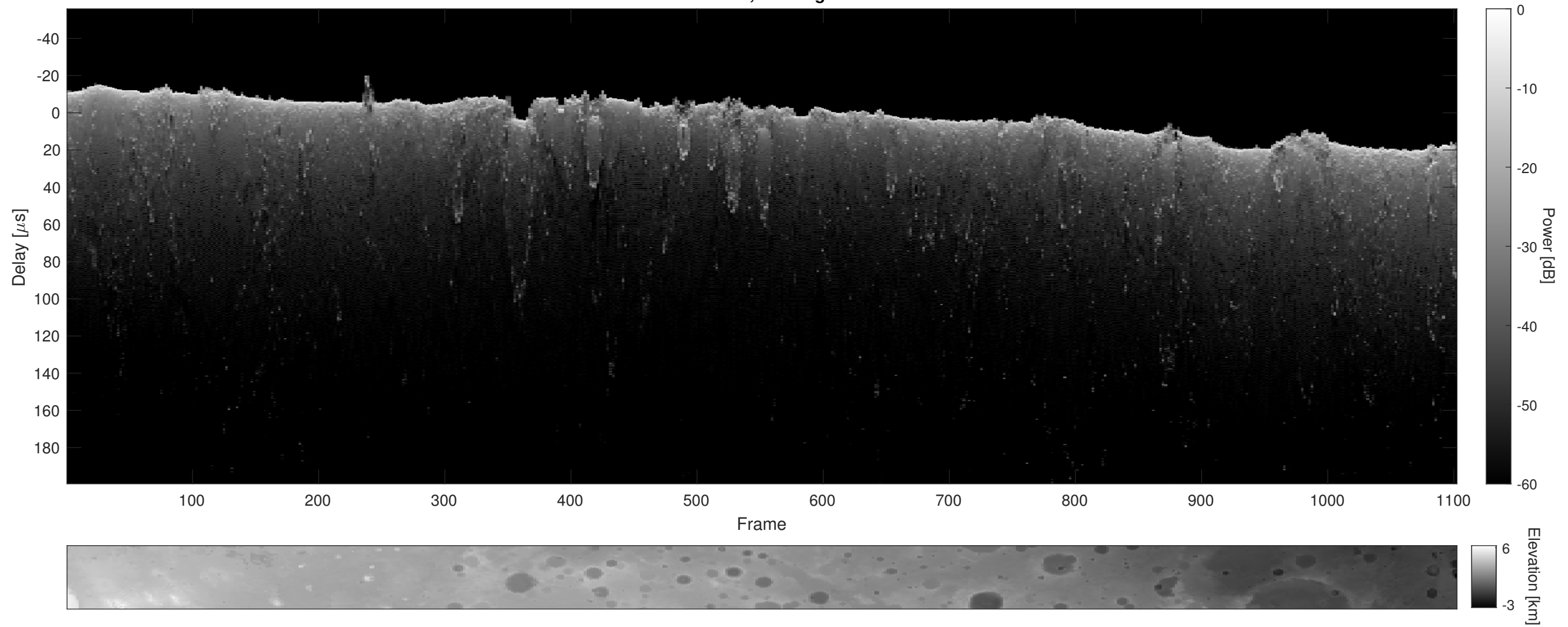
Orbit 2258, Cluttergram
