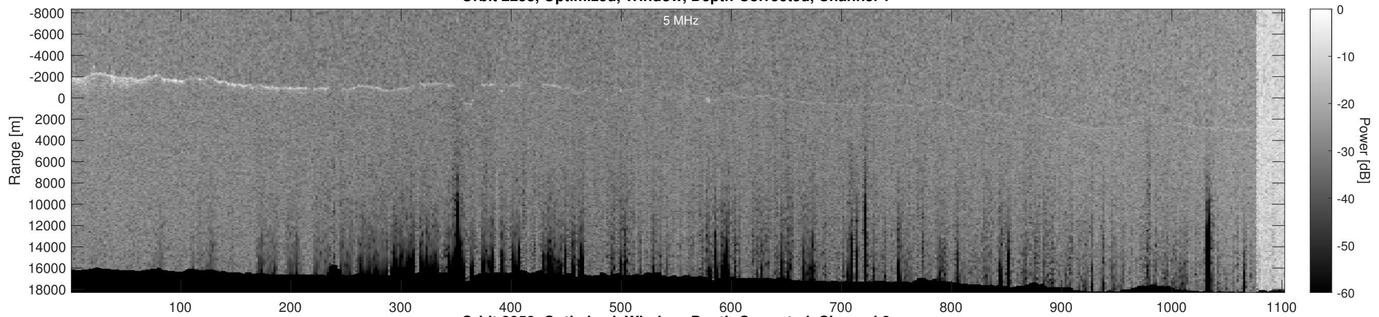
Orbit 2258, Optimized, Window, Depth-Corrected, Channel 2
