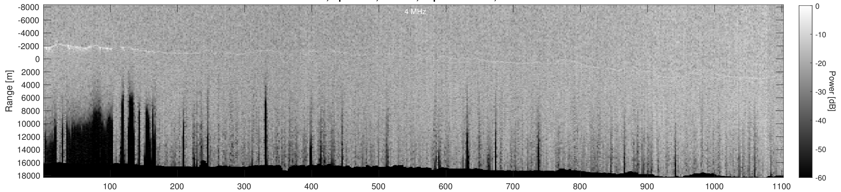
Orbit 2258, Depth-Corrected Cluttergram
