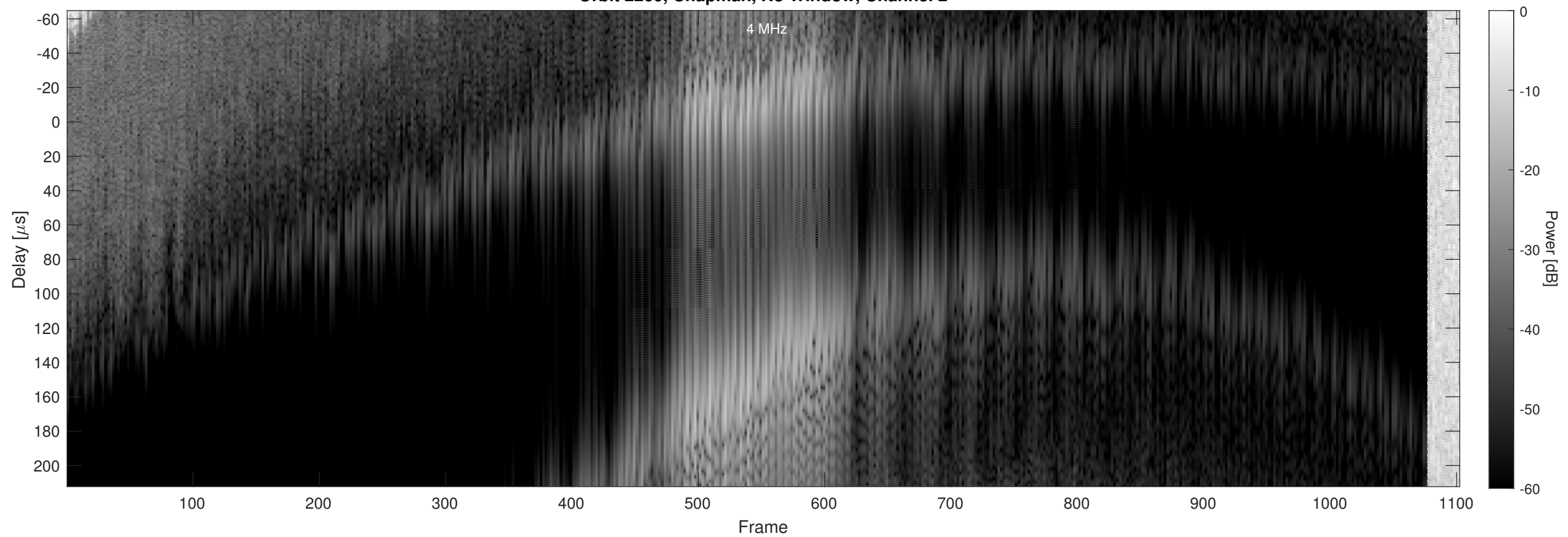
Orbit 2260, Chapman, No Window, Channel 2
