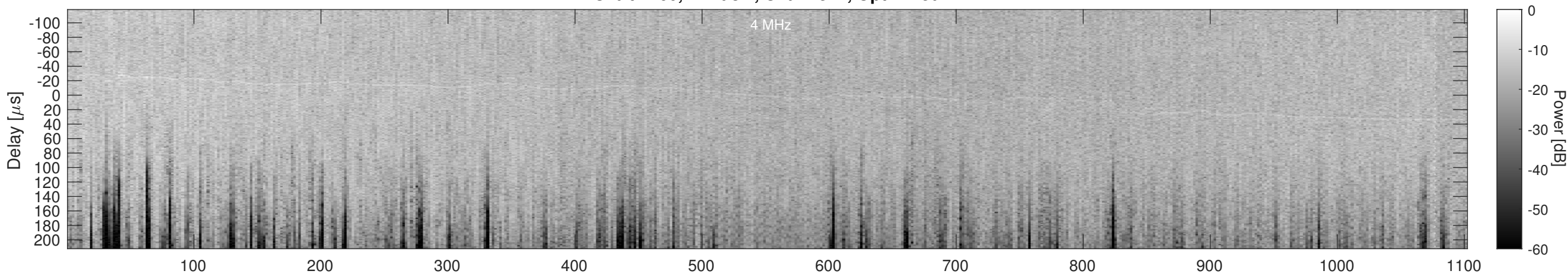
Orbit 2260, Cluttergram
