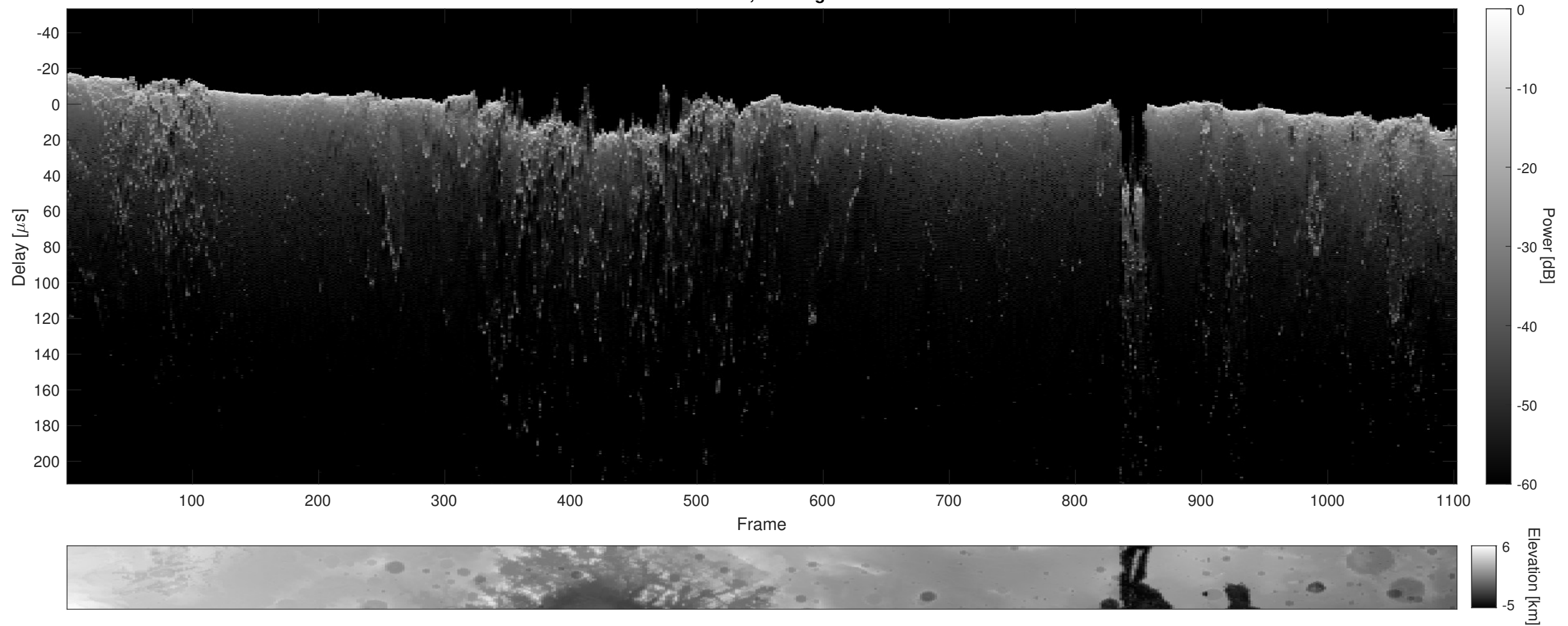
Orbit 2266, Cluttergram
