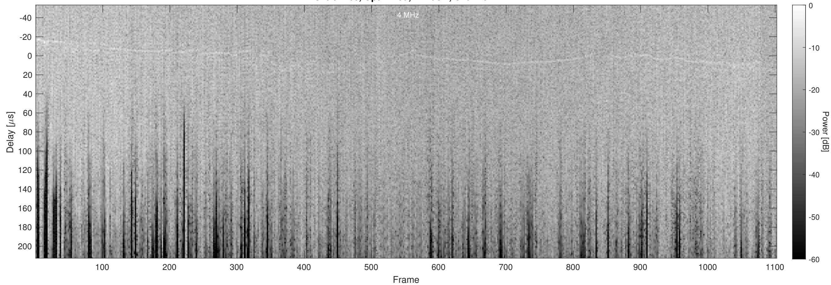
Orbit 2266, Optimized, Window, Channel 2
