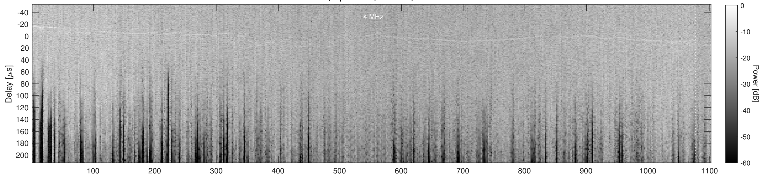
Orbit 2266, Cluttergram
