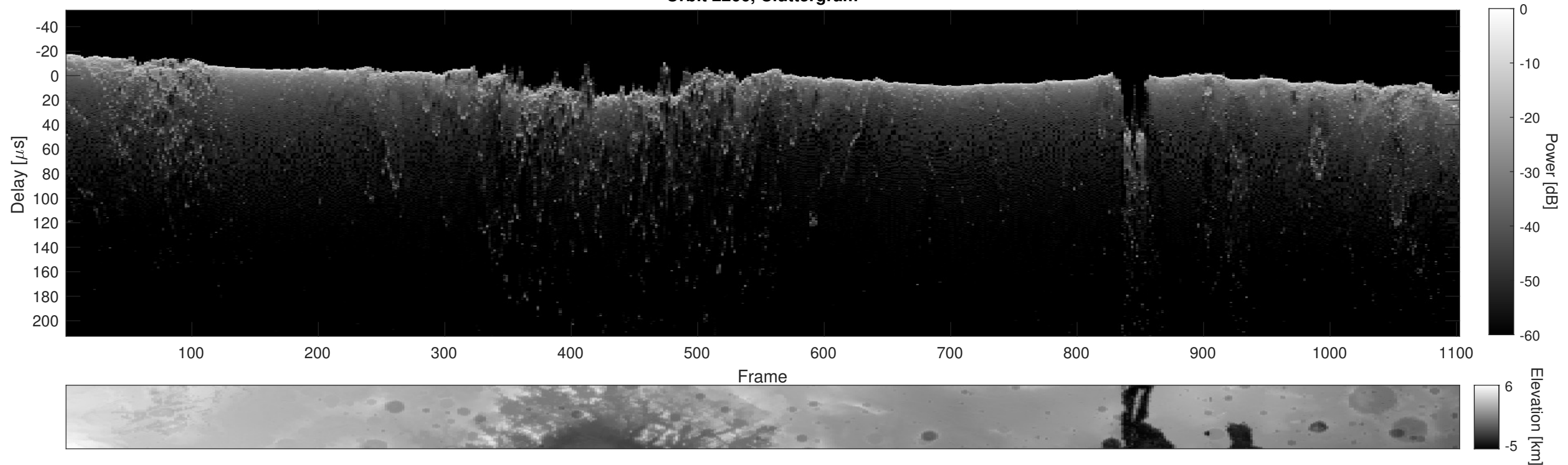
Orbit 2266, Cluttergram
