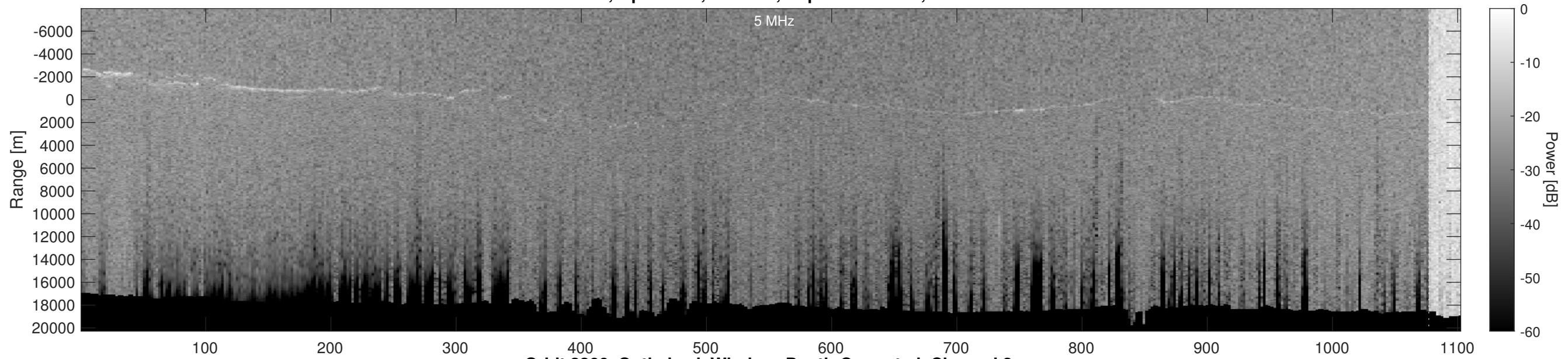
Orbit 2266, Optimized, Window, Depth-Corrected, Channel 2
