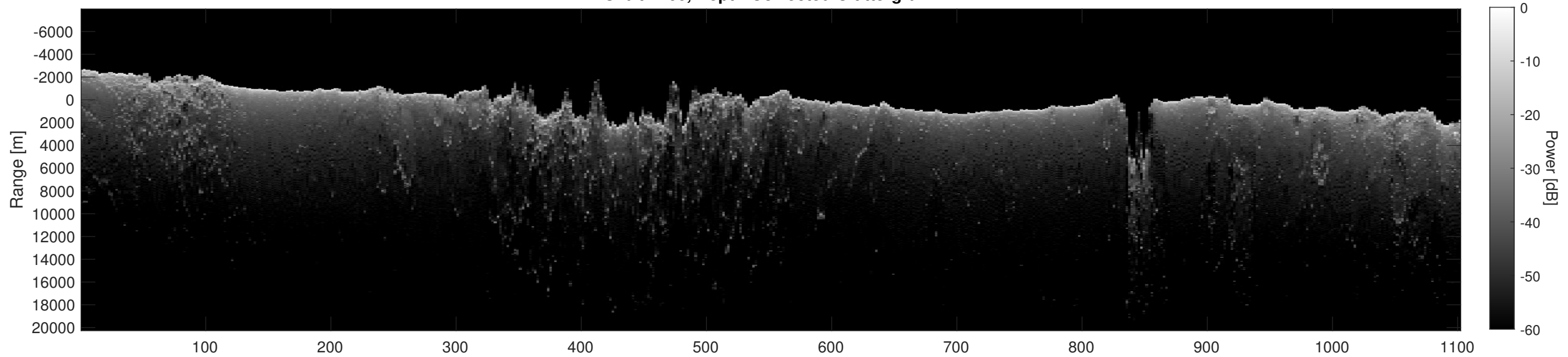
Orbit 2266, Depth-Corrected Cluttergram
