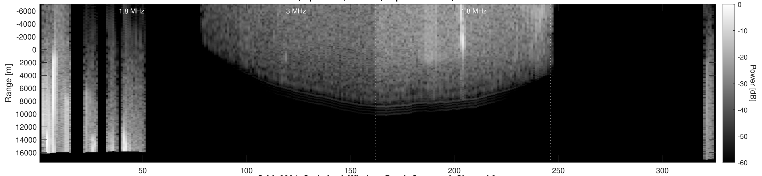
Orbit 2304, Optimized, Window, Depth-Corrected, Channel 2
