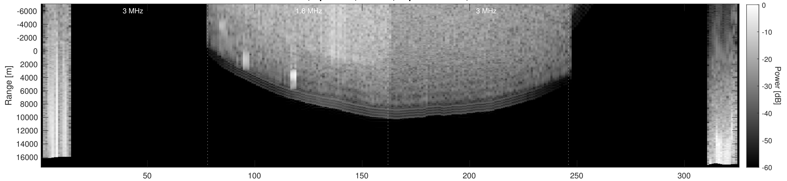
Orbit 2304, Depth-Corrected Cluttergram
