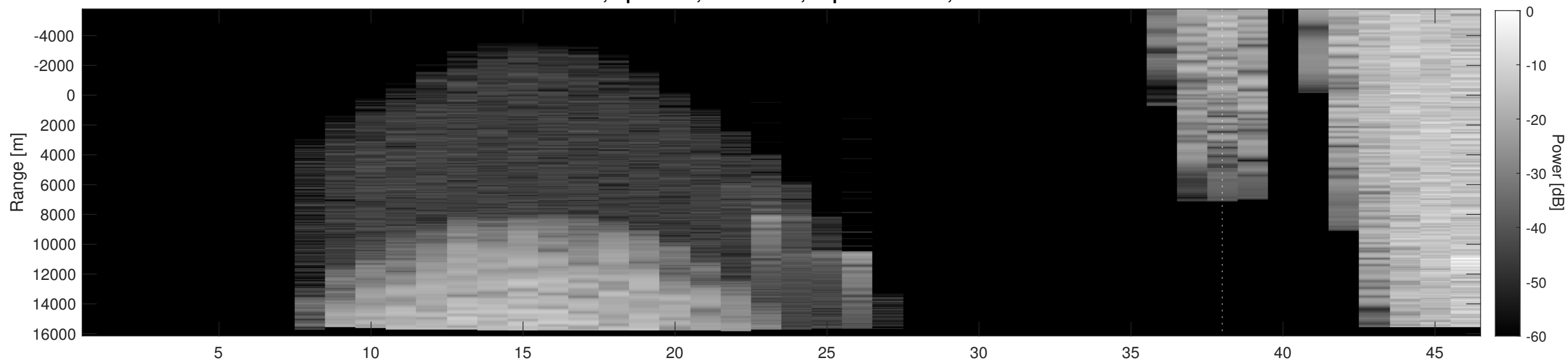
Orbit 2323, Depth-Corrected Cluttergram
