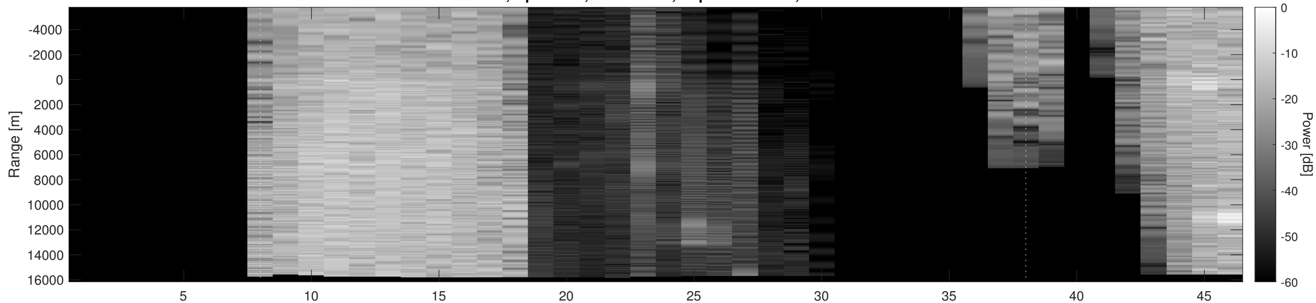
Orbit 2323, Optimized, No Window, Depth-Corrected, Channel 2
