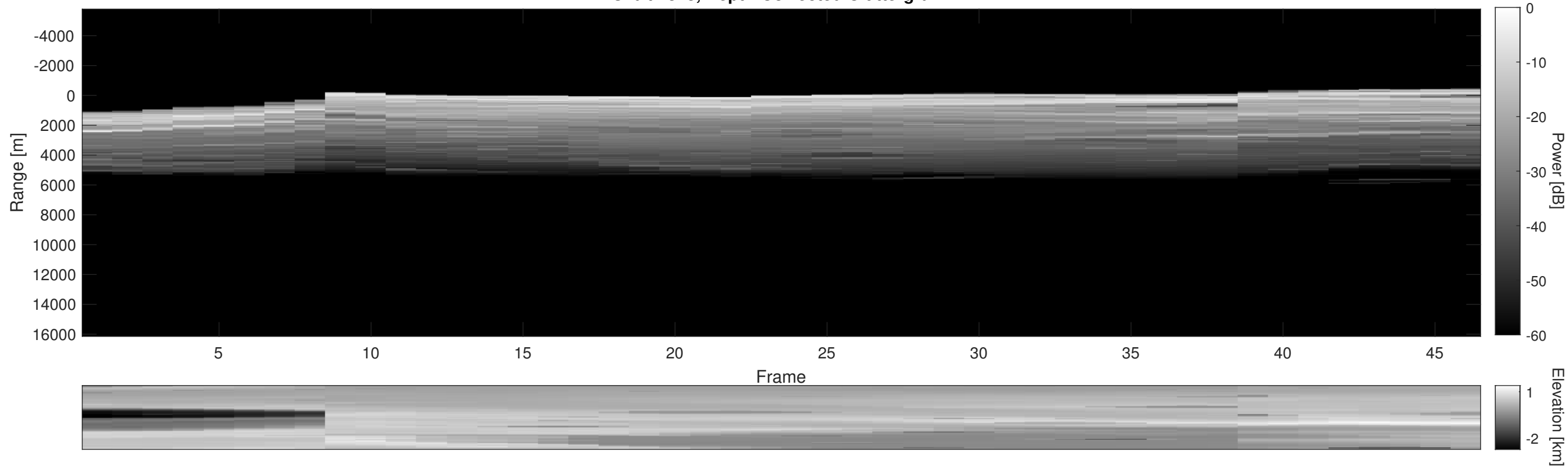
Orbit 2323, Depth-Corrected Cluttergram
