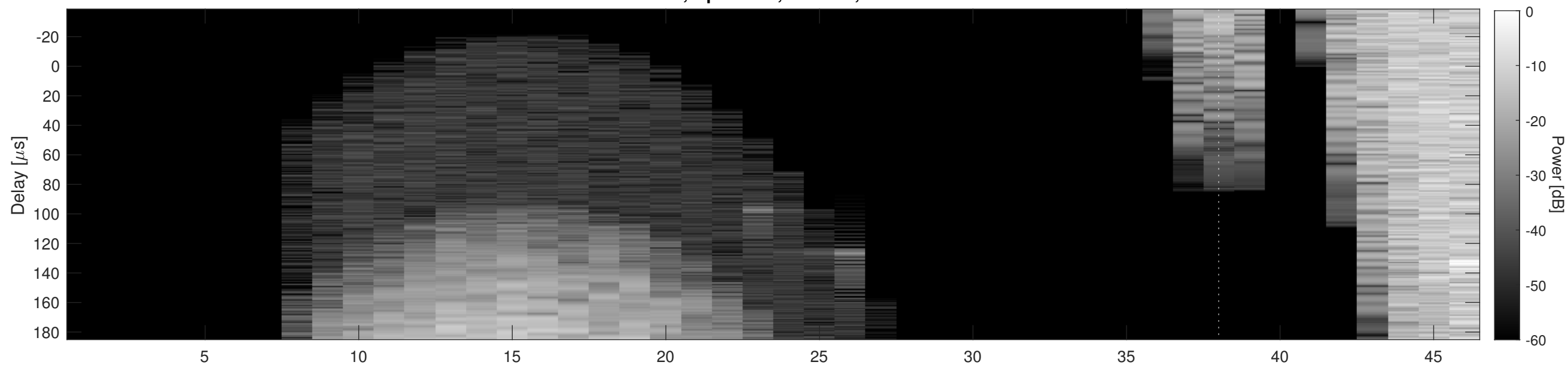
Orbit 2323, Cluttergram
