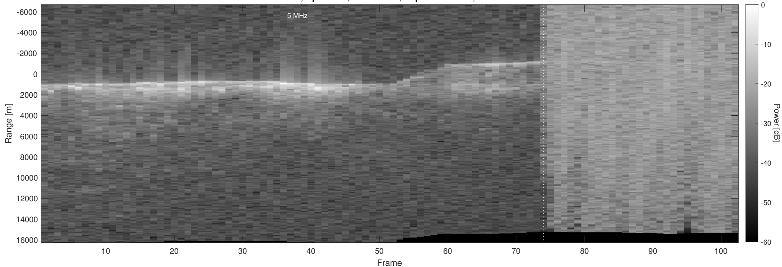
Orbit 2341, Optimized, No Window, Depth-Corrected, Channel 2
