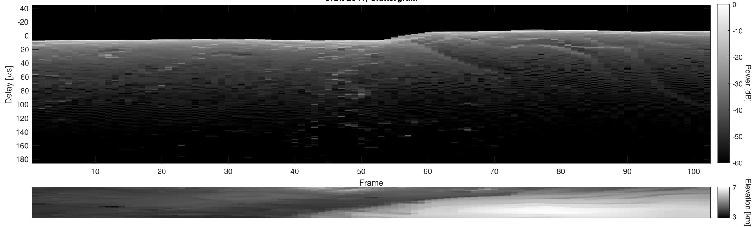
Orbit 2341, Cluttergram
