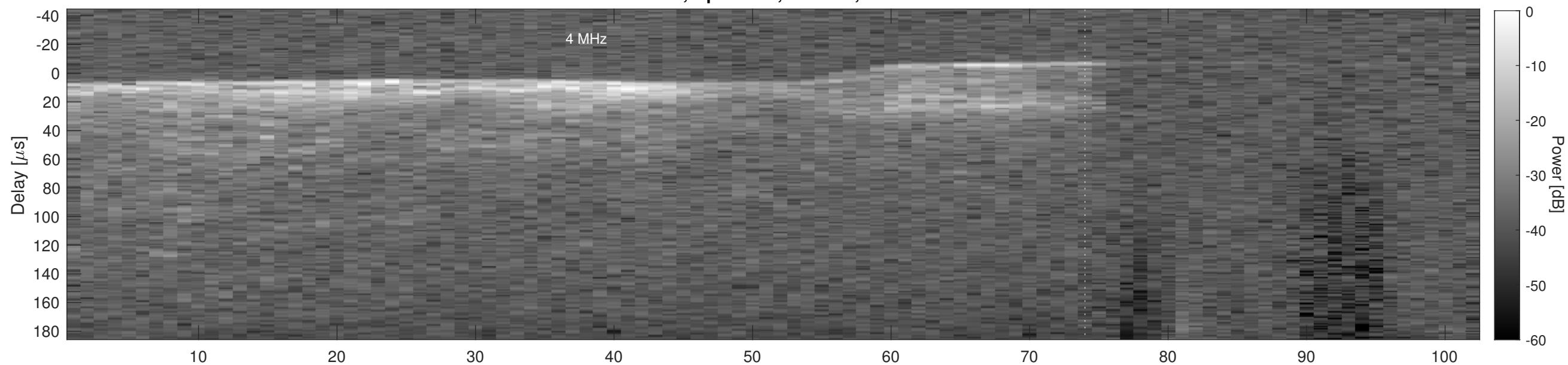
Orbit 2341, Cluttergram
