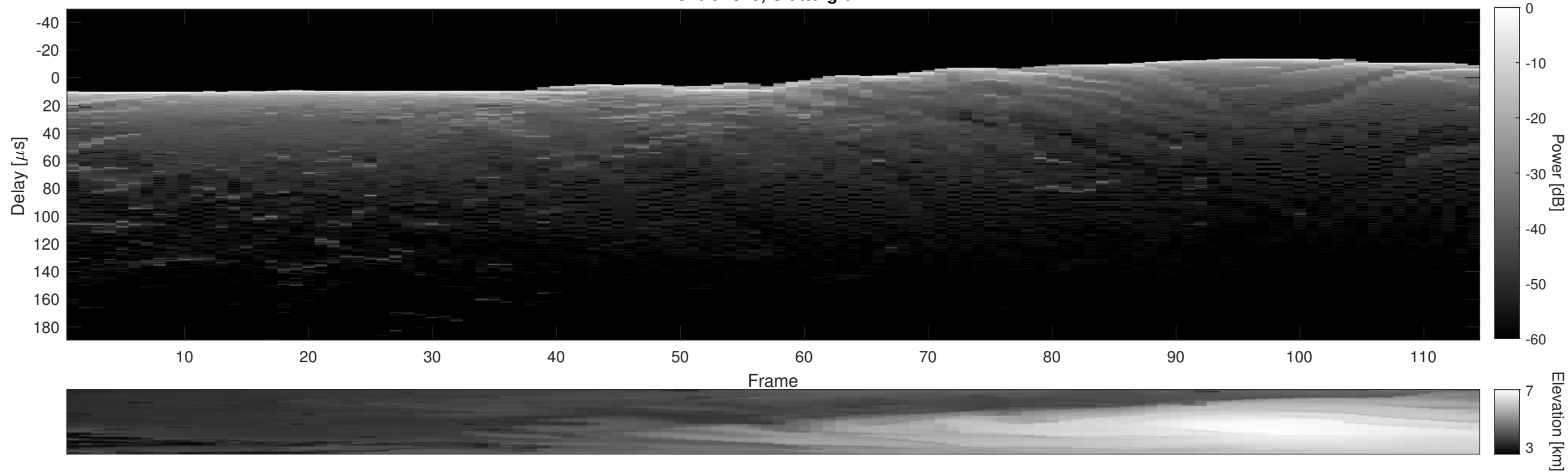
Orbit 2345, Cluttergram
