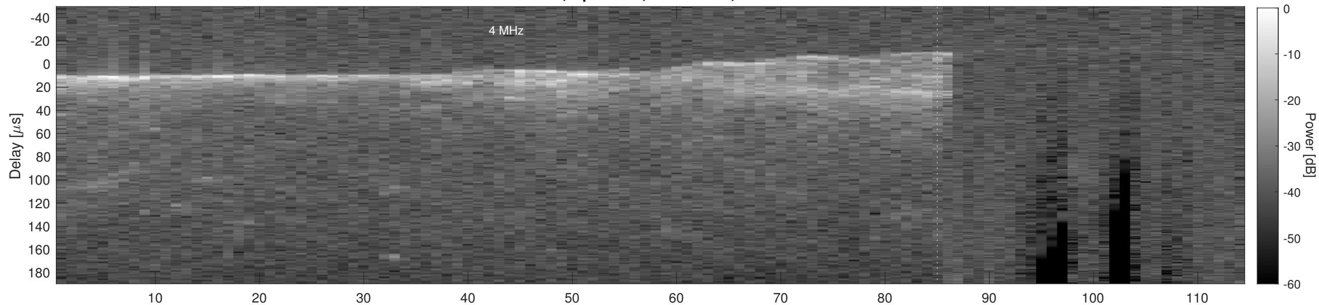
Orbit 2345, Cluttergram
