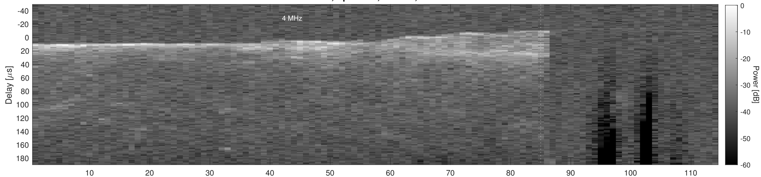
Orbit 2345, Cluttergram
