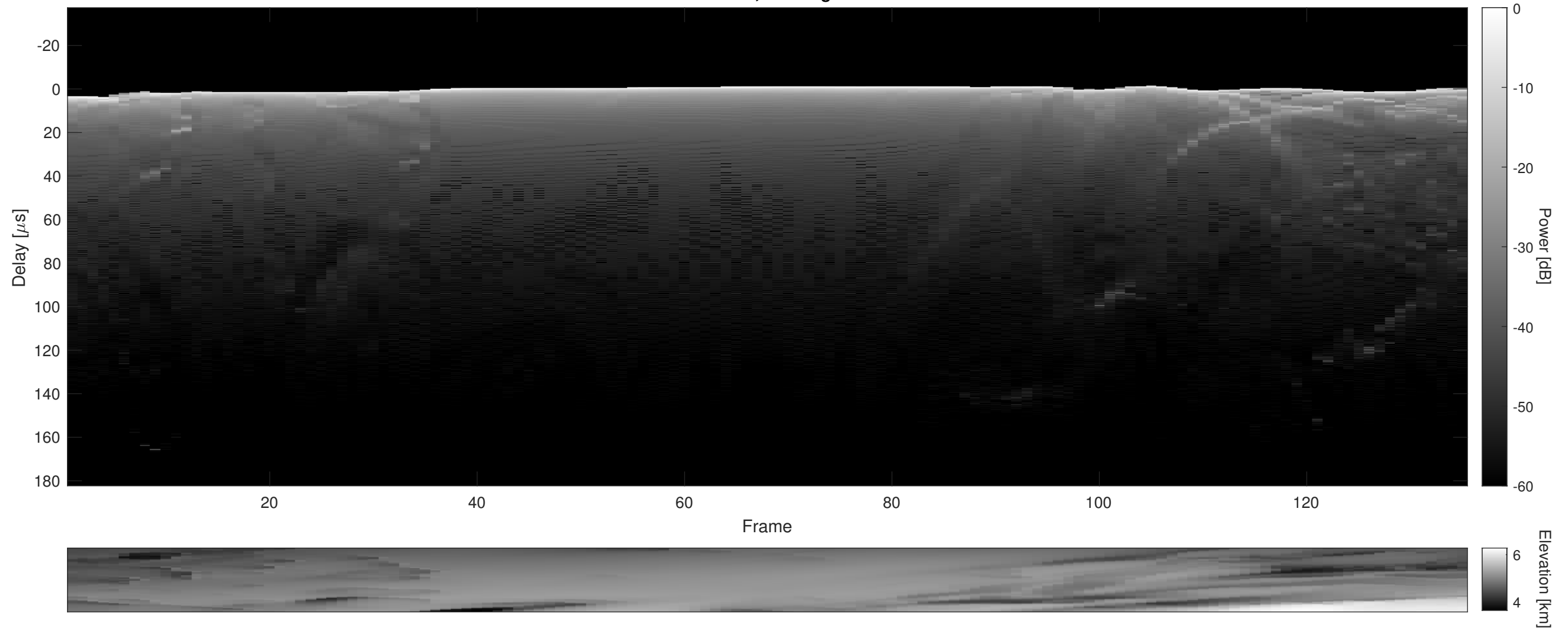
Orbit 2350, Cluttergram
