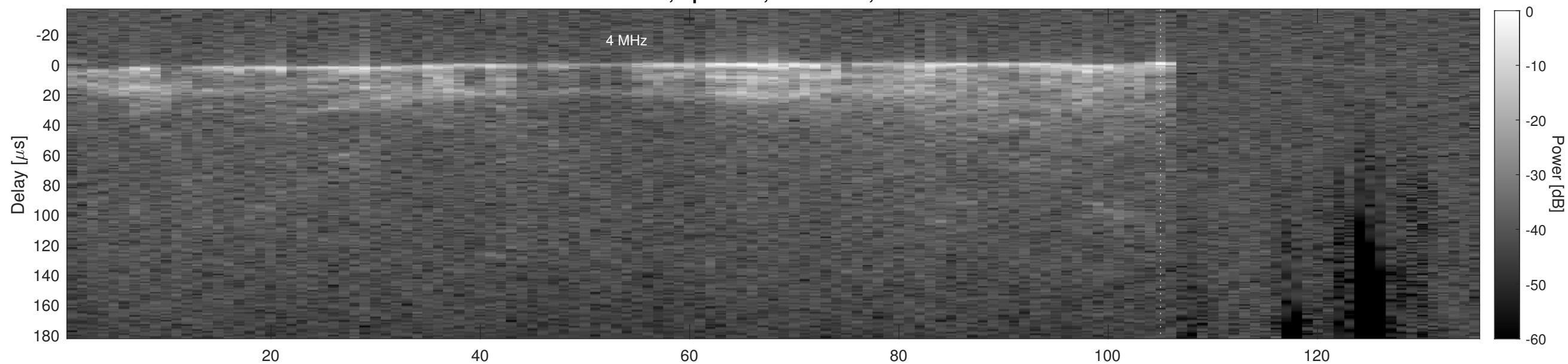
Orbit 2350, Cluttergram
