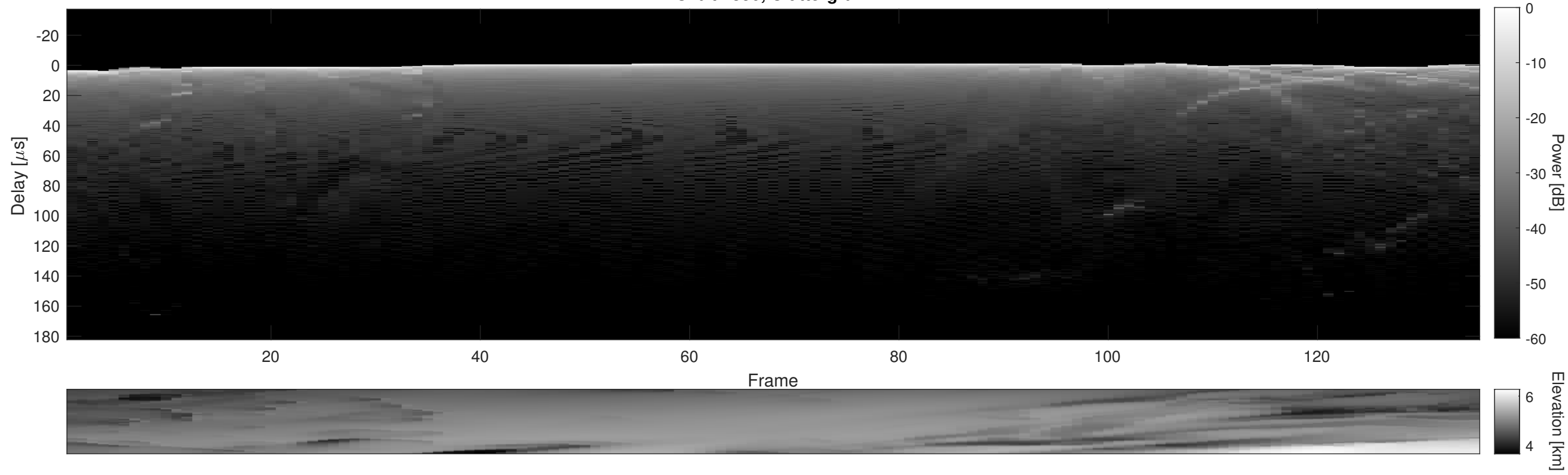
Orbit 2350, Cluttergram
