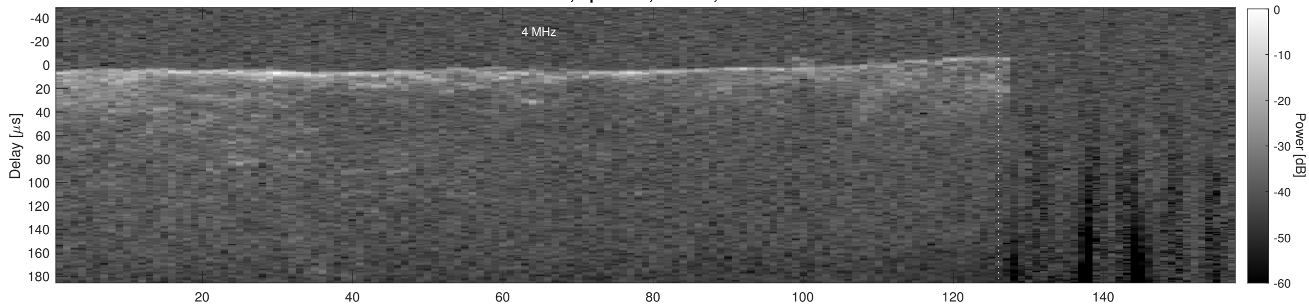
Orbit 2360, Cluttergram
