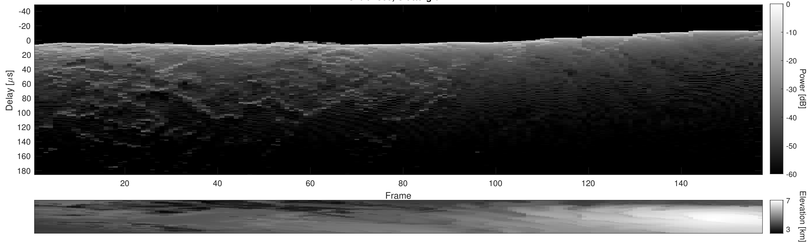
Orbit 2360, Cluttergram
