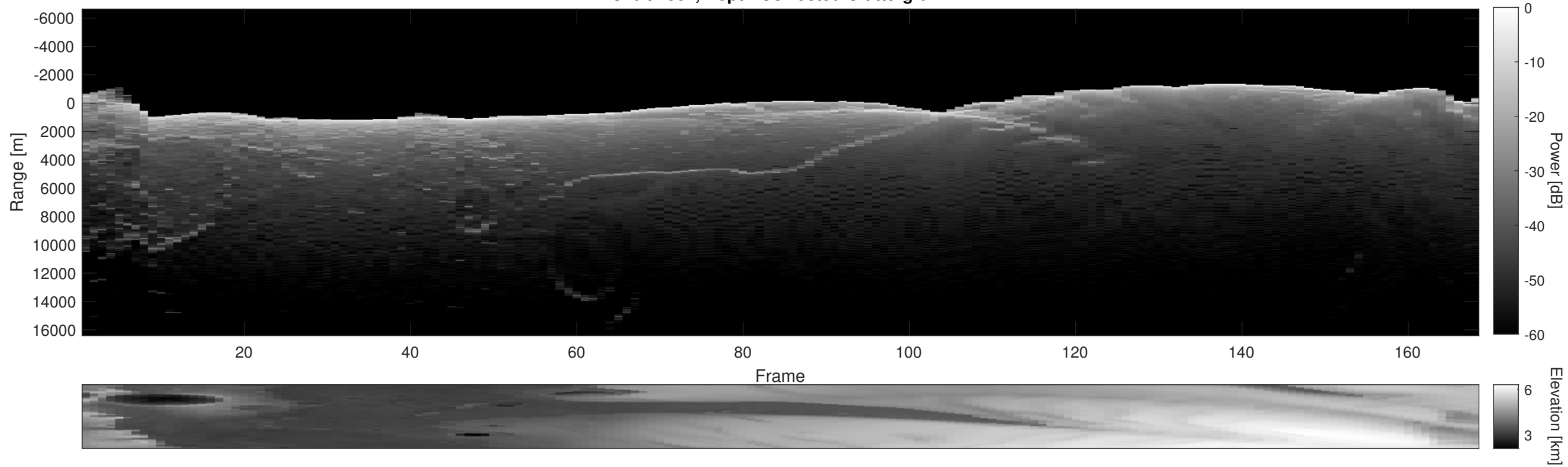
Orbit 2362, Depth-Corrected Cluttergram
