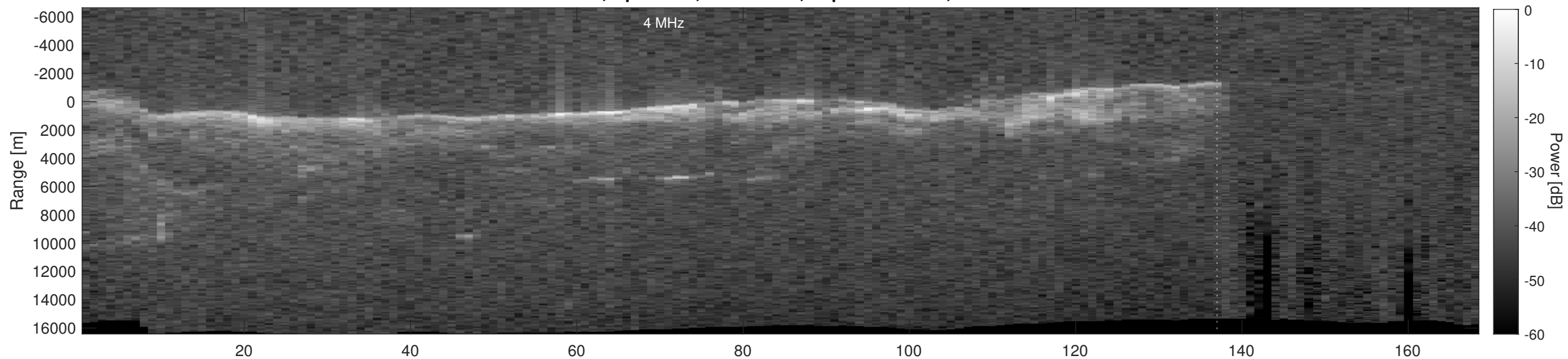
Orbit 2362, Depth-Corrected Cluttergram
