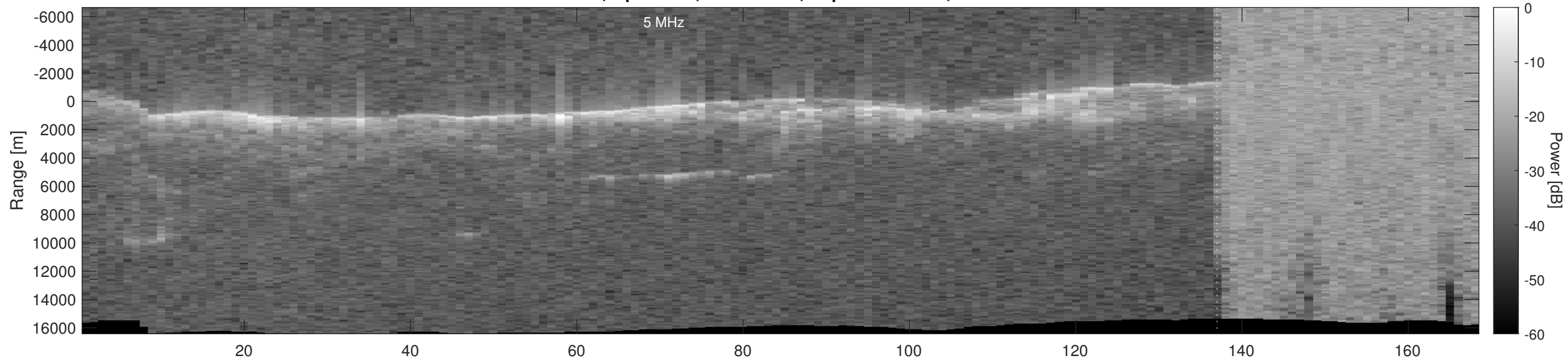
Orbit 2362, Optimized, No Window, Depth-Corrected, Channel 2
