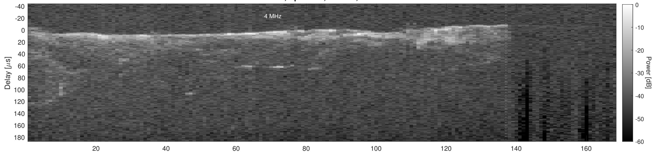
Orbit 2362, Cluttergram
