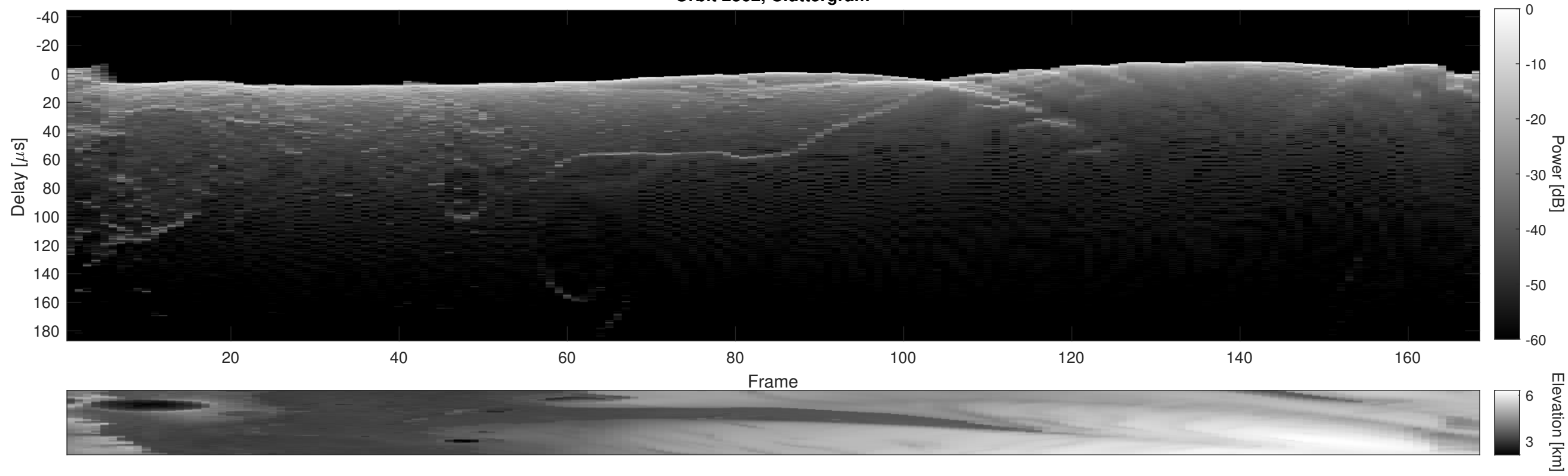
Orbit 2362, Cluttergram
